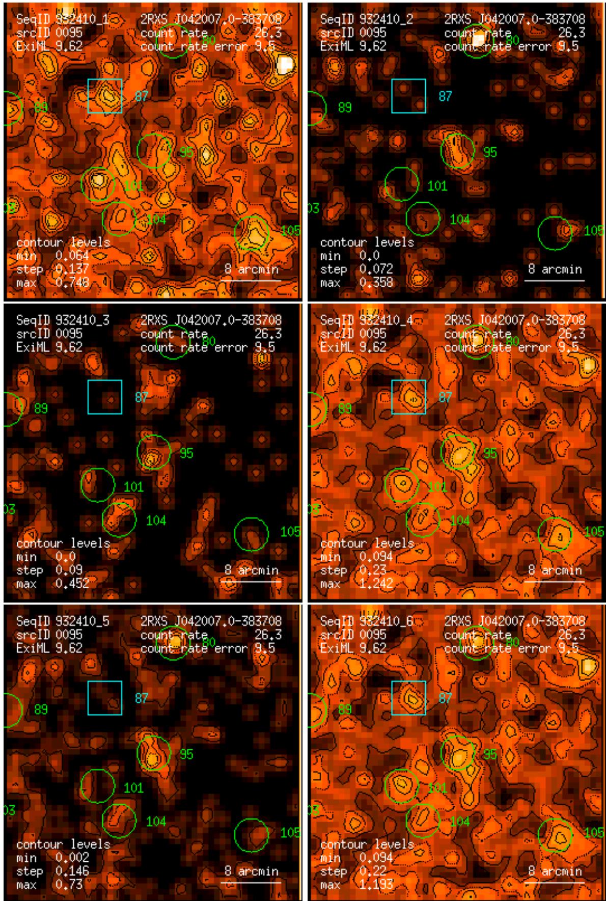
Figure 95: RASS 932410: detection 0095: band rate images, Gaussian filter: (1) PSPC channels 11 – 41, (2) 52 – 90, (3) 91 – 201, (4) 11 – 235, (5) 52 – 201, (6) 11 – 201. Broad band rates in counts/ks. Band rate contour levels in counts/ks/arcmin 2 .
