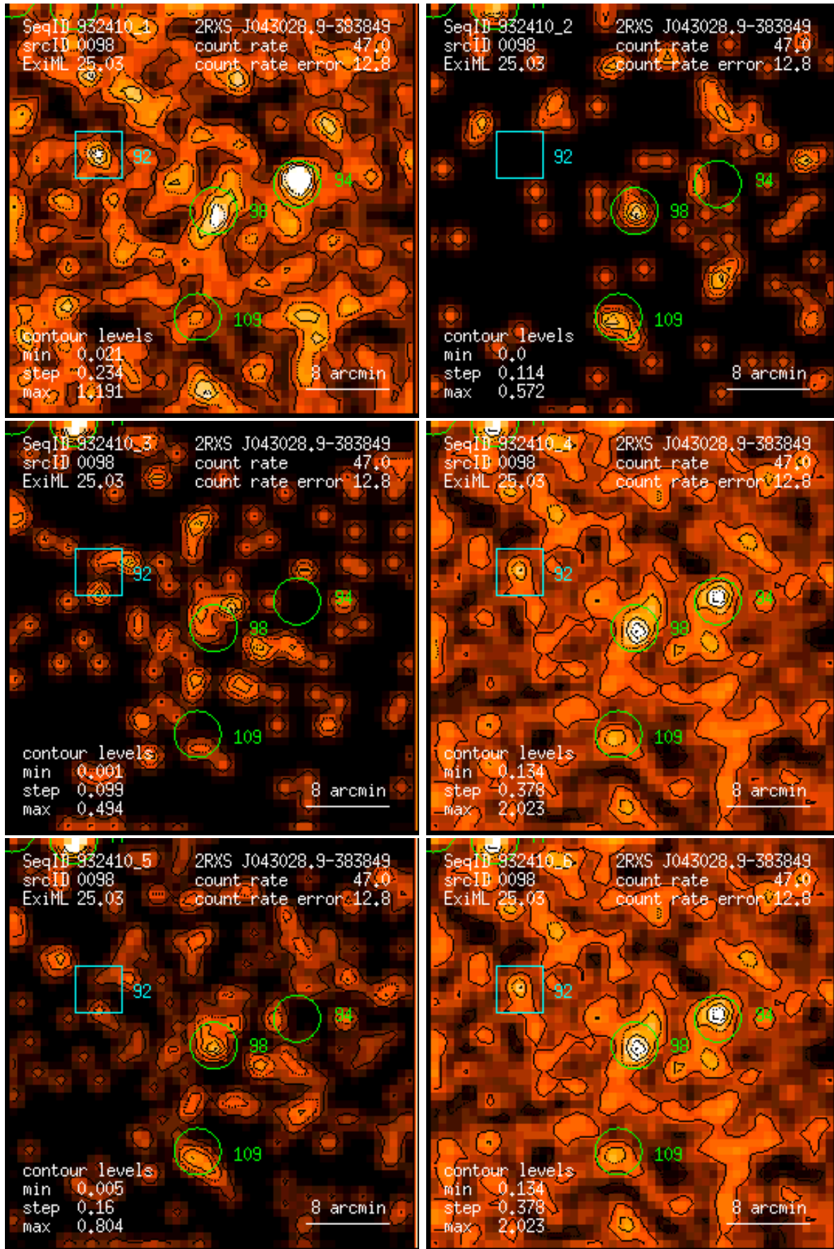
Figure 98: RASS 932410: detection 0098: band rate images, Gaussian filter: (1) PSPC channels 11 – 41, (2) 52 – 90, (3) 91 – 201, (4) 11 – 235, (5) 52 – 201, (6) 11 – 201. Broad band rates in counts/ks. Band rate contour levels in counts/ks/arcmin 2 .
