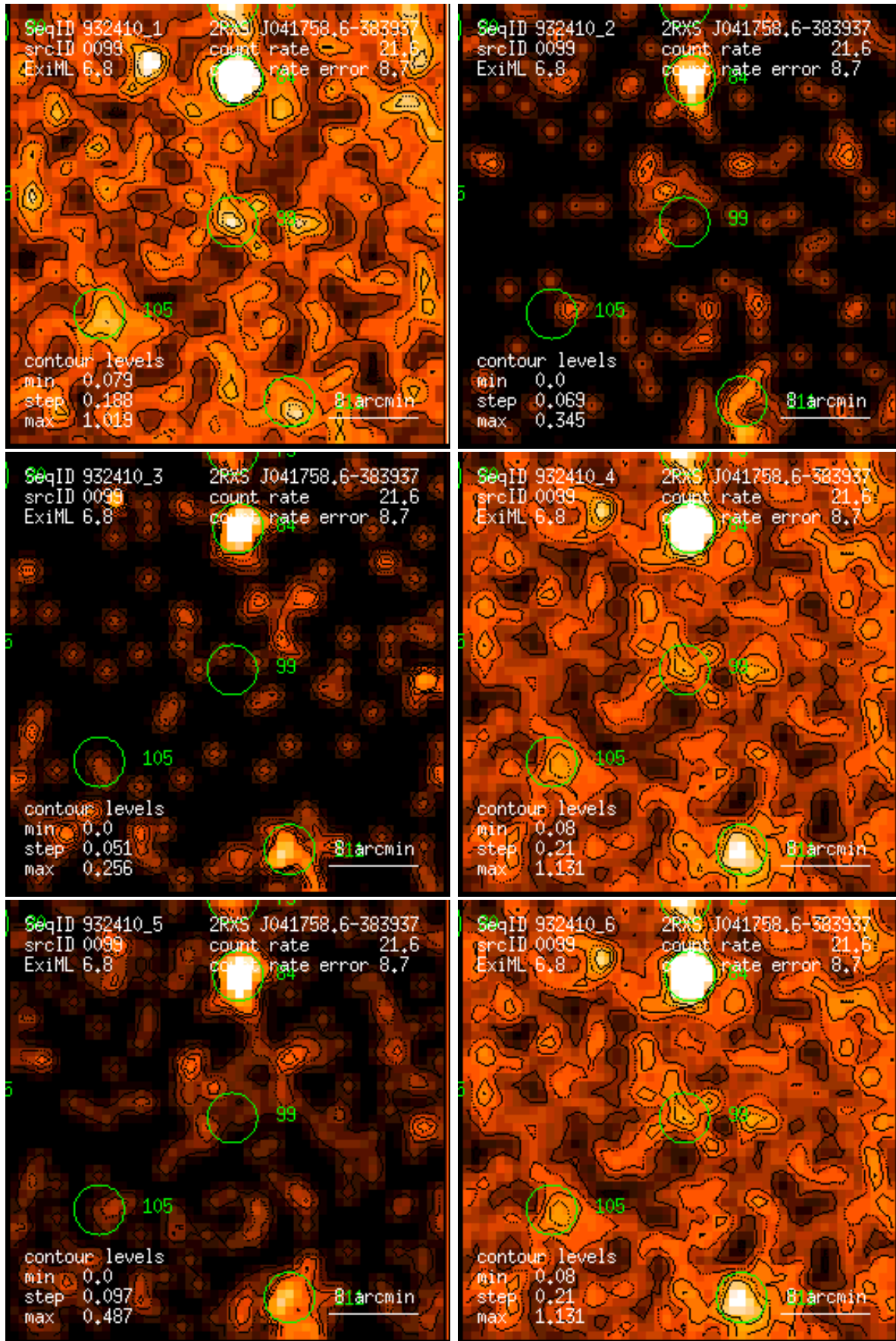
Figure 99: RASS 932410: detection 0099: band rate images, Gaussian filter: (1) PSPC channels 11 – 41, (2) 52 – 90, (3) 91 – 201, (4) 11 – 235, (5) 52 – 201, (6) 11 – 201. Broad band rates in counts/ks. Band rate contour levels in counts/ks/arcmin 2 .
