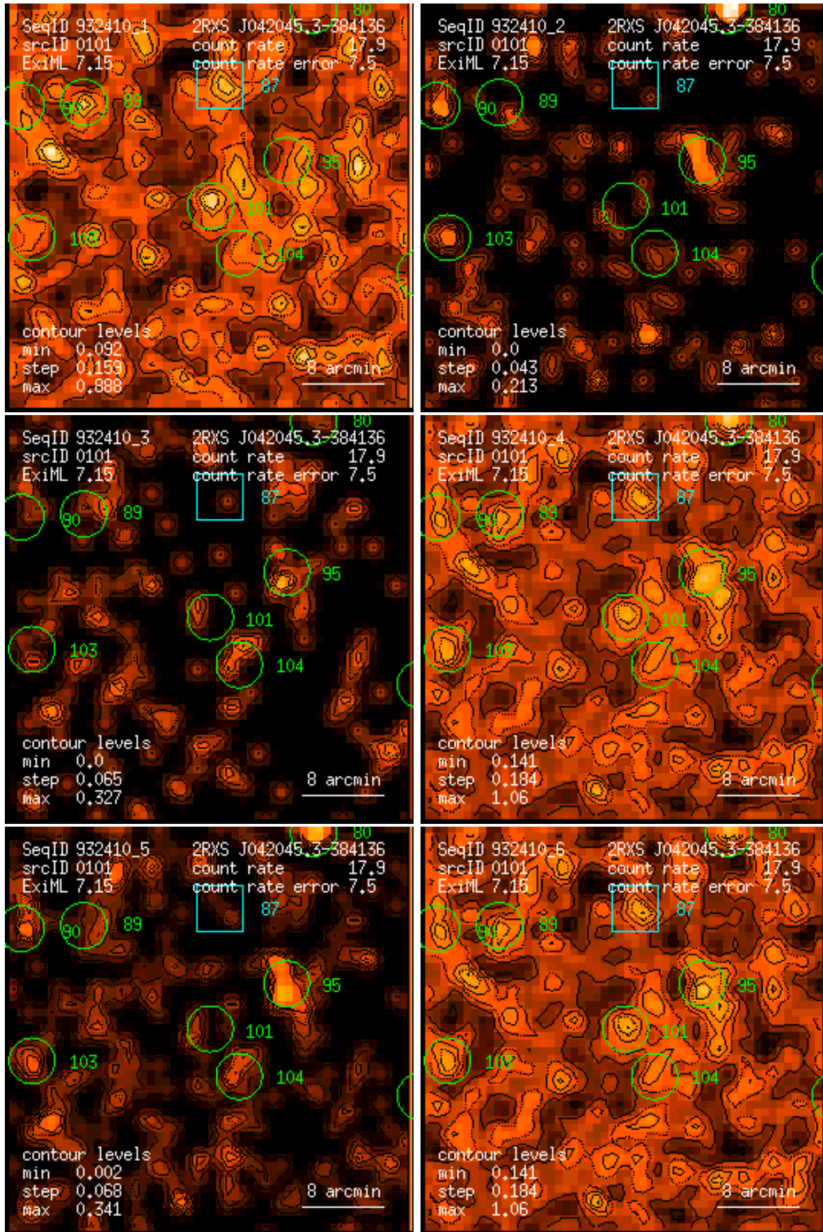
Figure 101: RASS 932410: detection 0101: band rate images, Gaussian filter: (1) PSPC channels 11 – 41, (2) 52 – 90, (3) 91 – 201, (4) 11 – 235, (5) 52 – 201, (6) 11 – 201. Broad band rates in counts/ks. Band rate contour levels in counts/ks/arcmin 2 .
