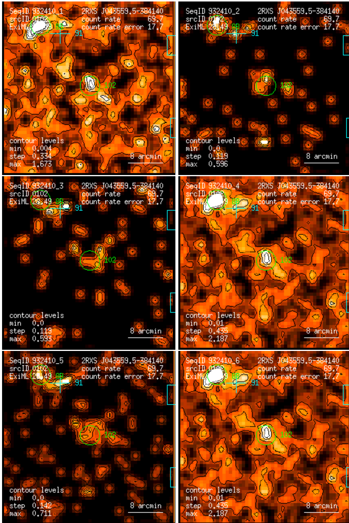
Figure 102: RASS 932410: detection 0102: band rate images, Gaussian filter: (1) PSPC channels 11 – 41, (2) 52 – 90, (3) 91 – 201, (4) 11 – 235, (5) 52 – 201, (6) 11 – 201. Broad band rates in counts/ks. Band rate contour levels in counts/ks/arcmin 2 .
