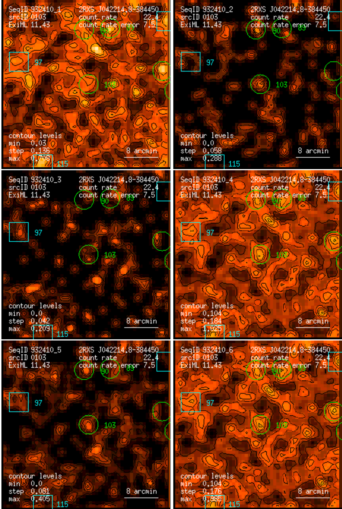
Figure 103: RASS 932410: detection 0103: band rate images, Gaussian filter: (1) PSPC channels 11 – 41, (2) 52 – 90, (3) 91 – 201, (4) 11 – 235, (5) 52 – 201, (6) 11 – 201. Broad band rates in counts/ks. Band rate contour levels in counts/ks/arcmin 2 .
