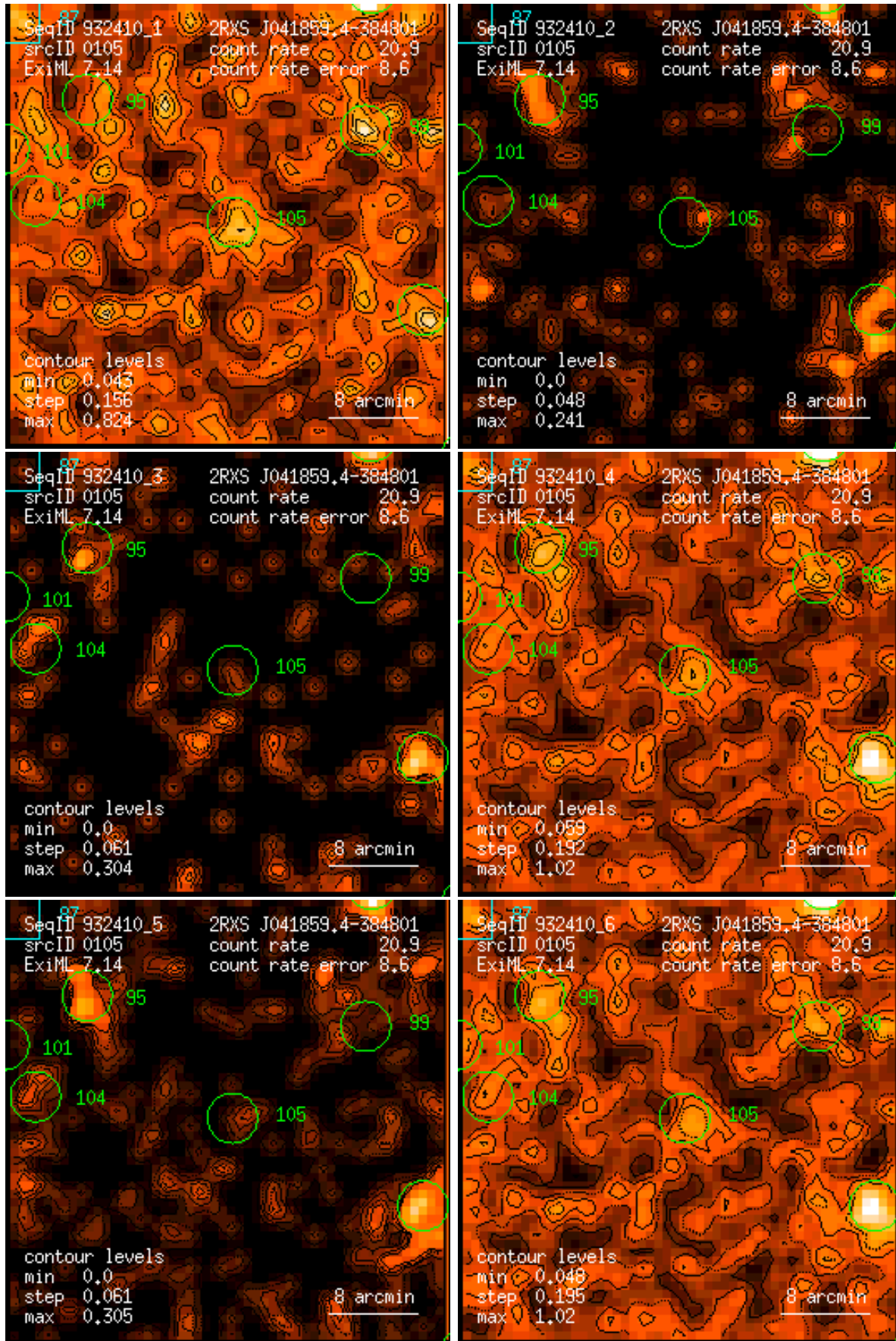
Figure 105: RASS 932410: detection 0105: band rate images, Gaussian filter: (1) PSPC channels 11 – 41, (2) 52 – 90, (3) 91 – 201, (4) 11 – 235, (5) 52 – 201, (6) 11 – 201. Broad band rates in counts/ks. Band rate contour levels in counts/ks/arcmin 2 .
