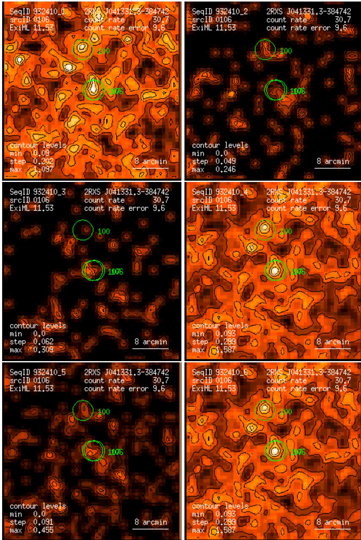
Figure 106: RASS 932410: detection 0106: band rate images, Gaussian filter: (1) PSPC channels 11 – 41, (2) 52 – 90, (3) 91 – 201, (4) 11 – 235, (5) 52 – 201, (6) 11 – 201. Broad band rates in counts/ks. Band rate contour levels in counts/ks/arcmin 2 .
