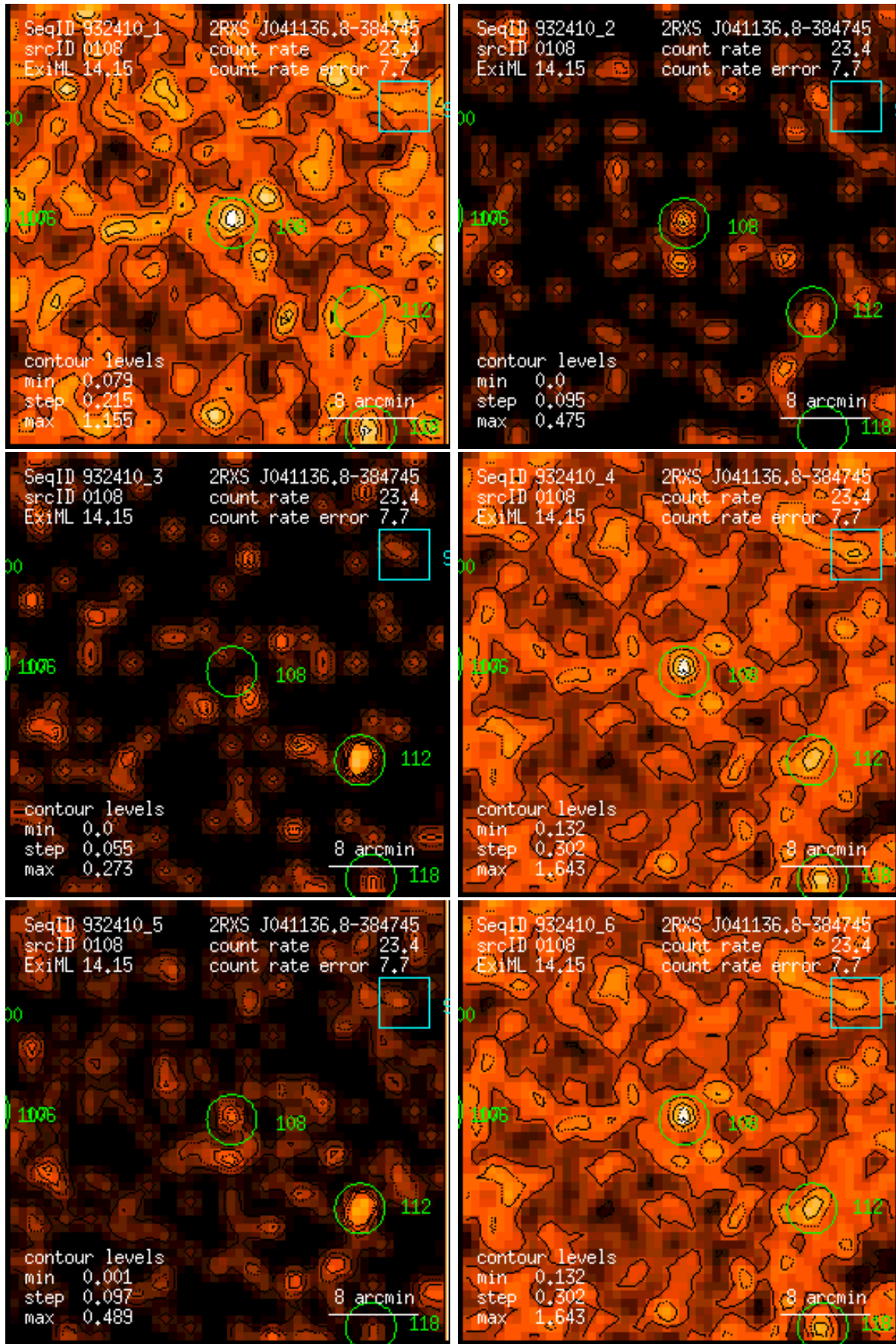
Figure 108: RASS 932410: detection 0108: band rate images, Gaussian filter: (1) PSPC channels 11 – 41, (2) 52 – 90, (3) 91 – 201, (4) 11 – 235, (5) 52 – 201, (6) 11 – 201. Broad band rates in counts/ks. Band rate contour levels in counts/ks/arcmin 2 .
