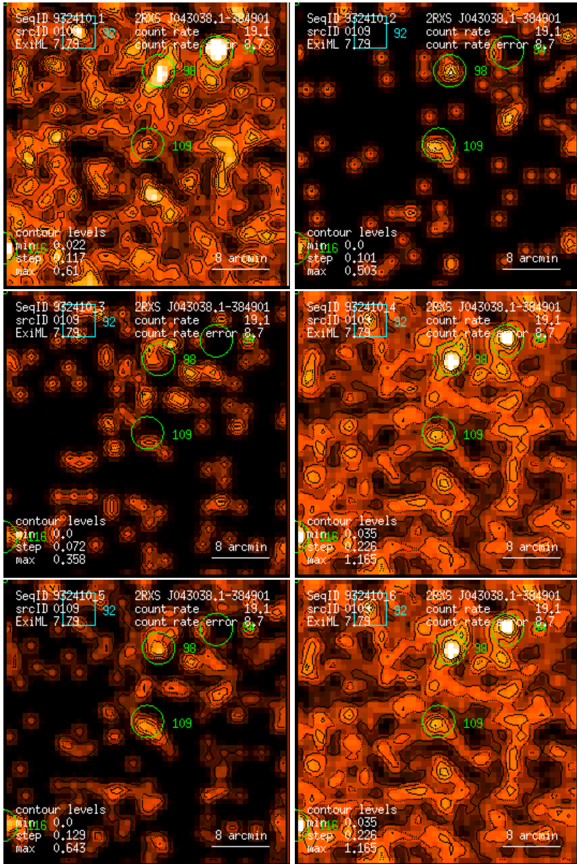
Figure 109: RASS 932410: detection 0109: band rate images, Gaussian filter: (1) PSPC channels 11 – 41, (2) 52 – 90, (3) 91 – 201, (4) 11 – 235, (5) 52 – 201, (6) 11 – 201. Broad band rates in counts/ks. Band rate contour levels in counts/ks/arcmin 2 .
