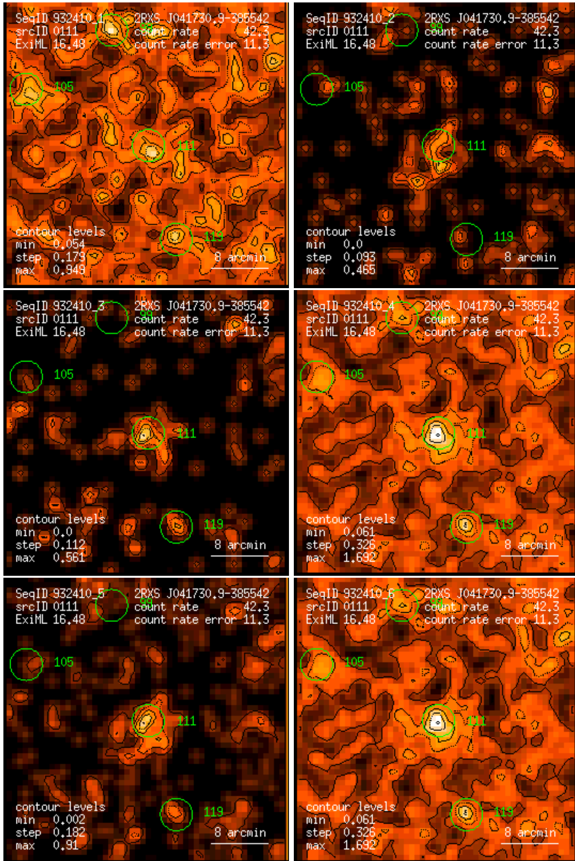
Figure 111: RASS 932410: detection 0111: band rate images, Gaussian filter: (1) PSPC channels 11 – 41, (2) 52 – 90, (3) 91 – 201, (4) 11 – 235, (5) 52 – 201, (6) 11 – 201. Broad band rates in counts/ks. Band rate contour levels in counts/ks/arcmin 2 .
