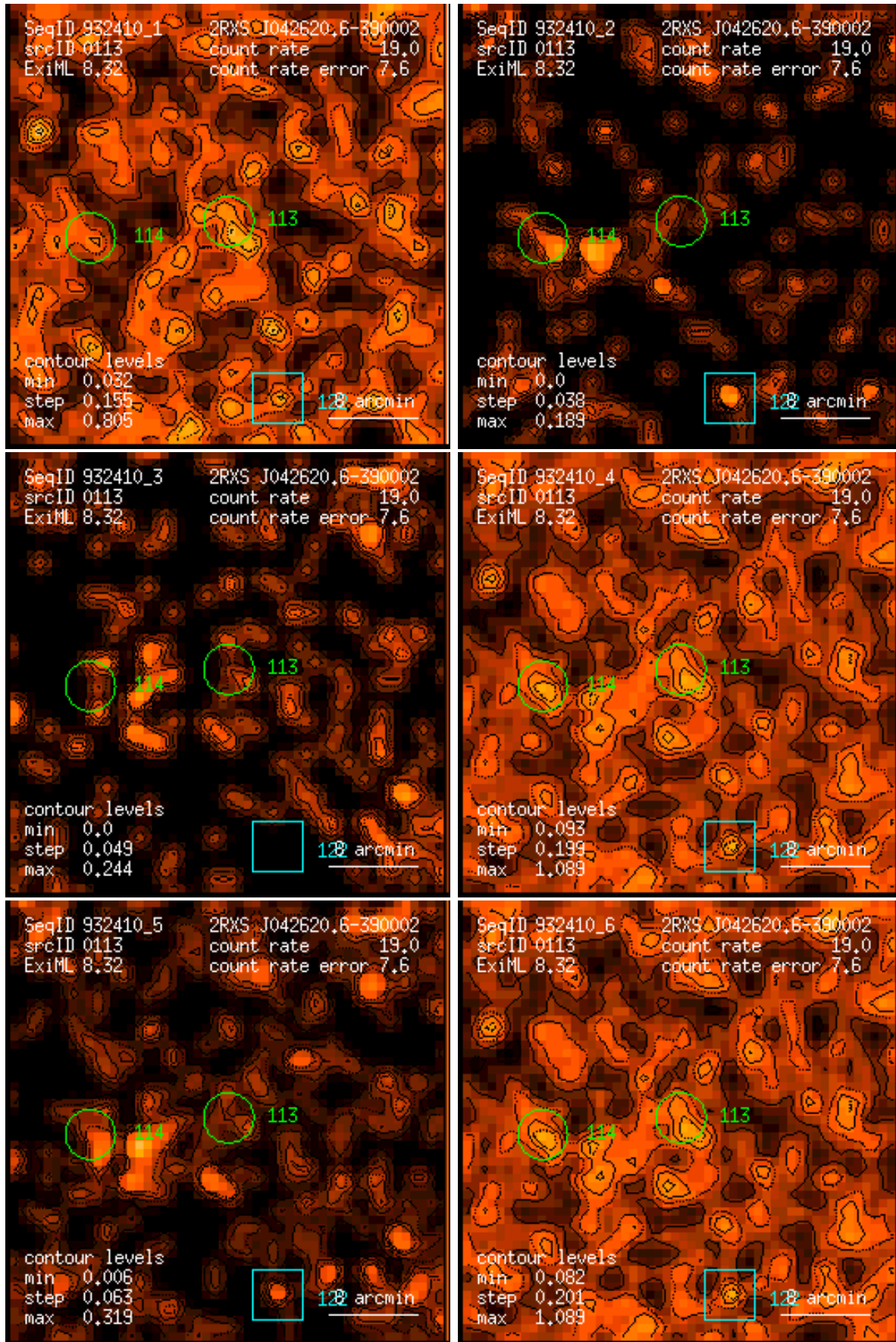
Figure 113: RASS 932410: detection 0113: band rate images, Gaussian filter: (1) PSPC channels 11 – 41, (2) 52 – 90, (3) 91 – 201, (4) 11 – 235, (5) 52 – 201, (6) 11 – 201. Broad band rates in counts/ks. Band rate contour levels in counts/ks/arcmin 2 .
