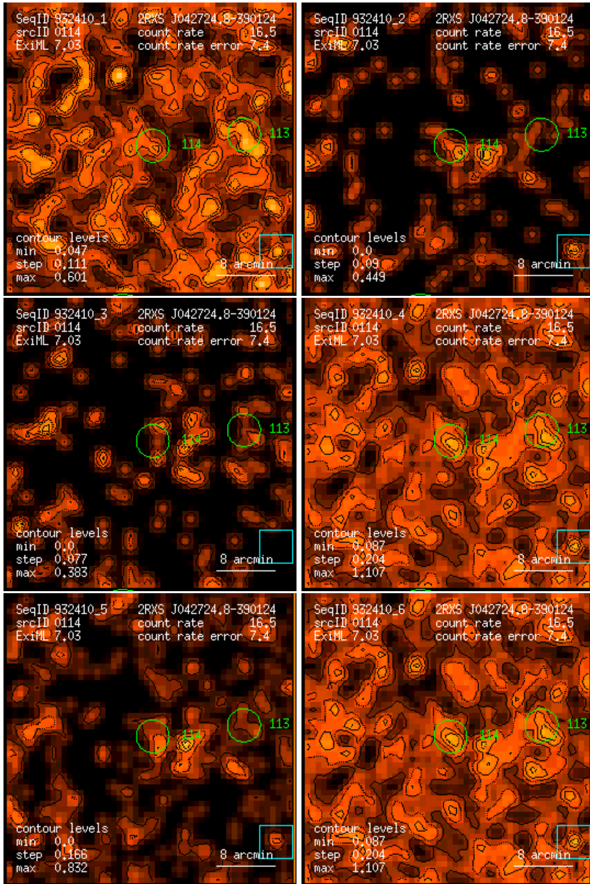
Figure 114: RASS 932410: detection 0114: band rate images, Gaussian filter: (1) PSPC channels 11 – 41, (2) 52 – 90, (3) 91 – 201, (4) 11 – 235, (5) 52 – 201, (6) 11 – 201. Broad band rates in counts/ks. Band rate contour levels in counts/ks/arcmin 2 .
