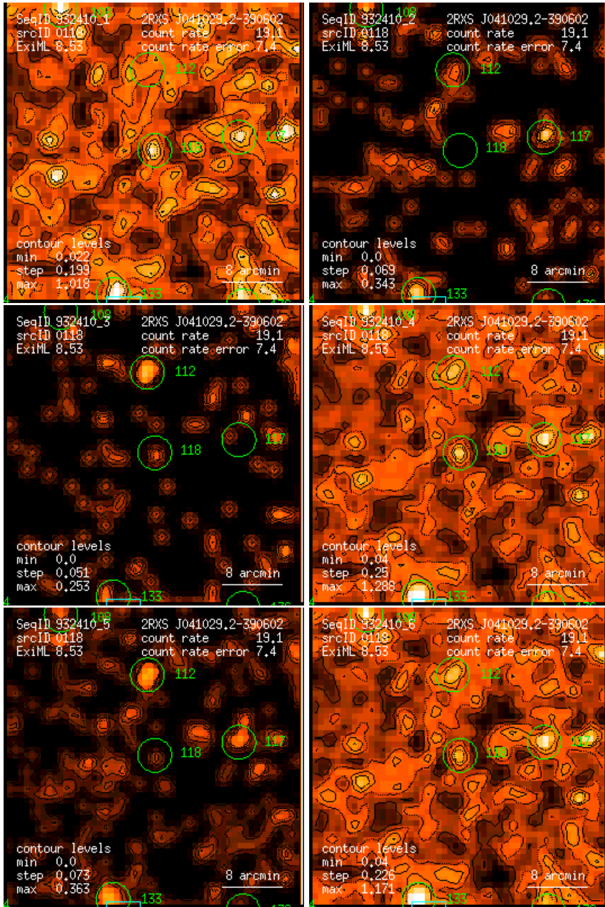
Figure 118: RASS 932410: detection 0118: band rate images, Gaussian filter: (1) PSPC channels 11 – 41, (2) 52 – 90, (3) 91 – 201, (4) 11 – 235, (5) 52 – 201, (6) 11 – 201. Broad band rates in counts/ks. Band rate contour levels in counts/ks/arcmin 2 .
