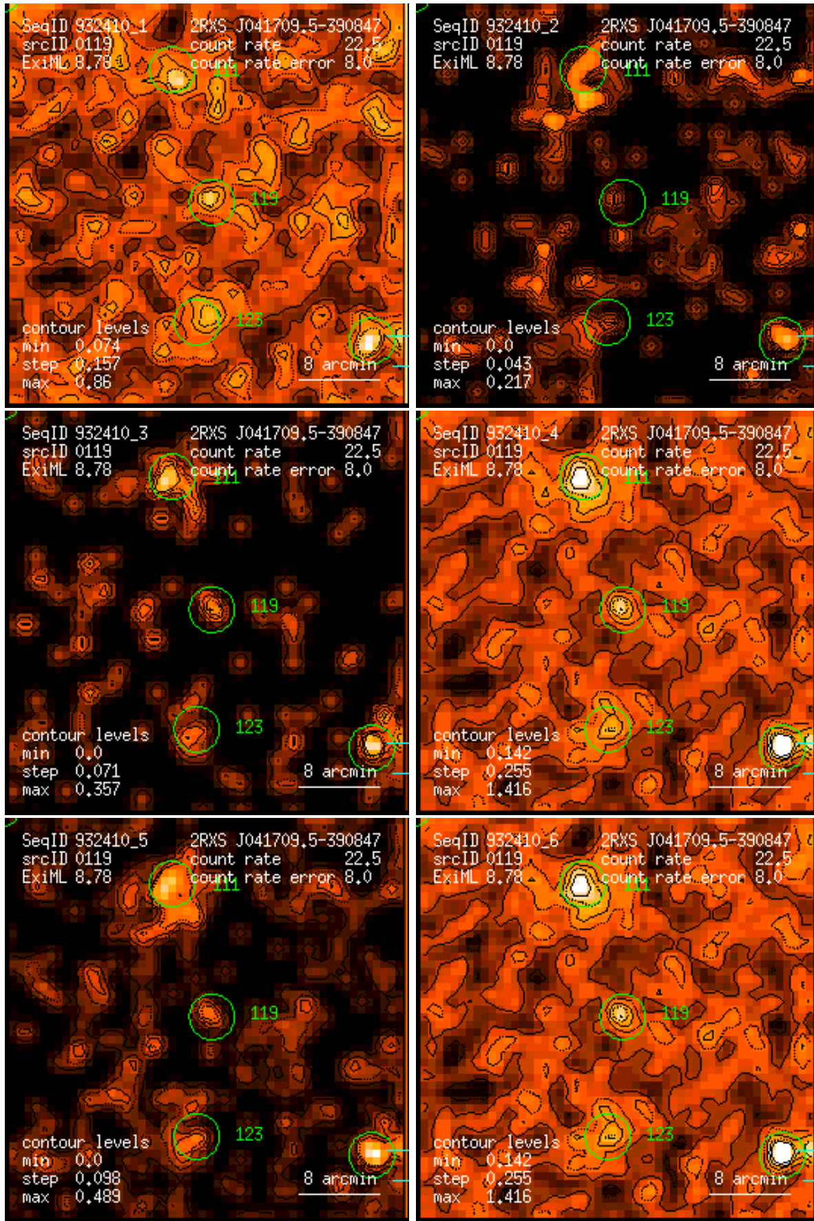
Figure 119: RASS 932410: detection 0119: band rate images, Gaussian filter: (1) PSPC channels 11 – 41, (2) 52 – 90, (3) 91 – 201, (4) 11 – 235, (5) 52 – 201, (6) 11 – 201. Broad band rates in counts/ks. Band rate contour levels in counts/ks/arcmin 2 .
