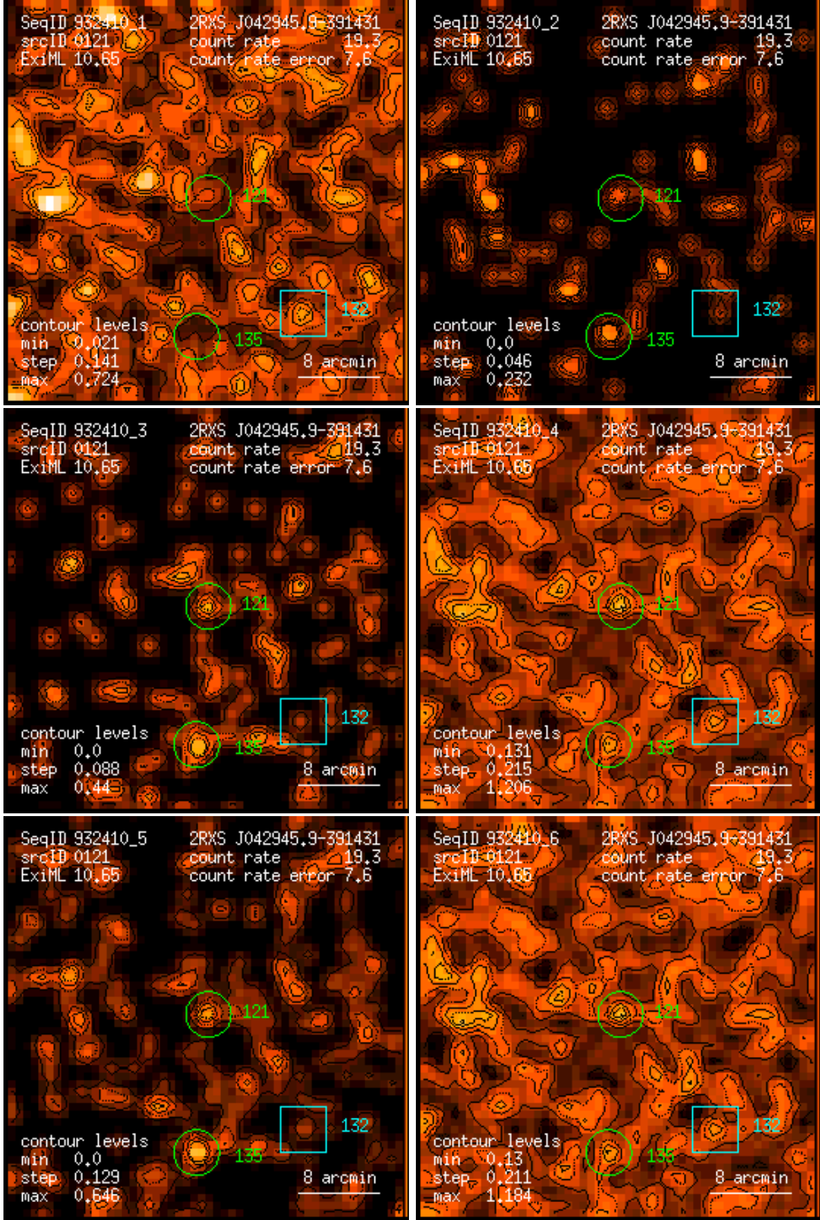
Figure 121: RASS 932410: detection 0121: band rate images, Gaussian filter: (1) PSPC channels 11 – 41, (2) 52 – 90, (3) 91 – 201, (4) 11 – 235, (5) 52 – 201, (6) 11 – 201. Broad band rates in counts/ks. Band rate contour levels in counts/ks/arcmin 2 .
