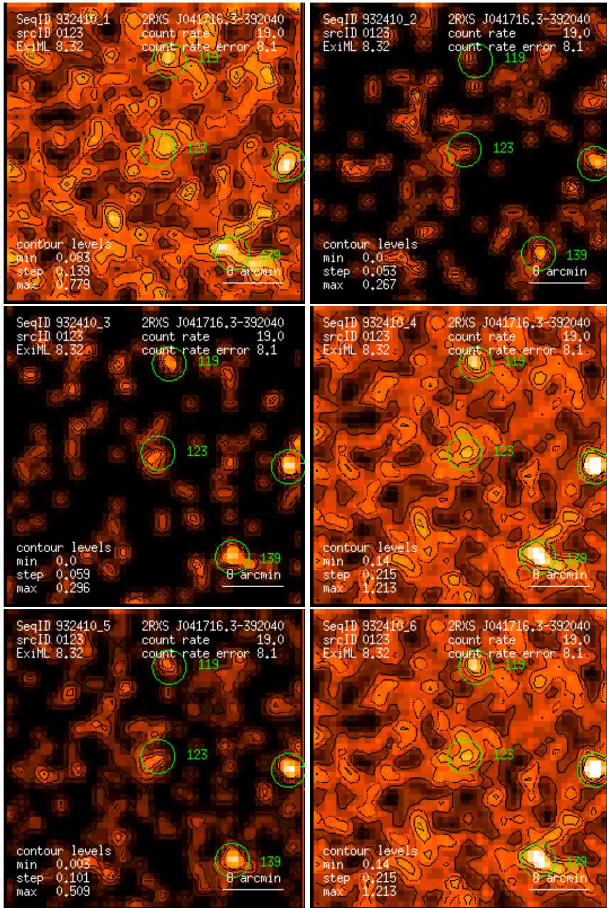
Figure 123: RASS 932410: detection 0123: band rate images, Gaussian filter: (1) PSPC channels 11 – 41, (2) 52 – 90, (3) 91 – 201, (4) 11 – 235, (5) 52 – 201, (6) 11 – 201. Broad band rates in counts/ks. Band rate contour levels in counts/ks/arcmin 2 .
