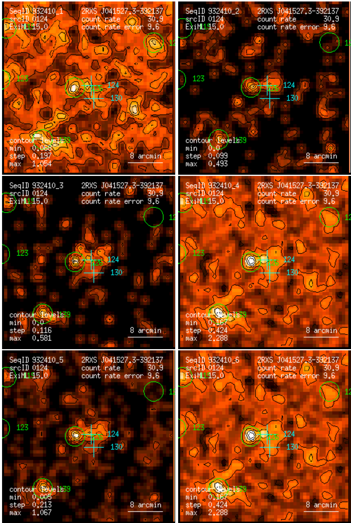
Figure 124: RASS 932410: detection 0124: band rate images, Gaussian filter: (1) PSPC channels 11 – 41, (2) 52 – 90, (3) 91 – 201, (4) 11 – 235, (5) 52 – 201, (6) 11 – 201. Broad band rates in counts/ks. Band rate contour levels in counts/ks/arcmin 2 .
