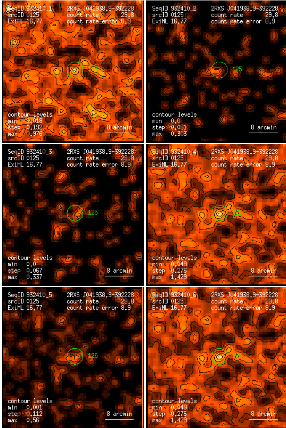
Figure 125: RASS 932410: detection 0125: band rate images, Gaussian filter: (1) PSPC channels 11 – 41, (2) 52 – 90, (3) 91 – 201, (4) 11 – 235, (5) 52 – 201, (6) 11 – 201. Broad band rates in counts/ks. Band rate contour levels in counts/ks/arcmin 2 .
