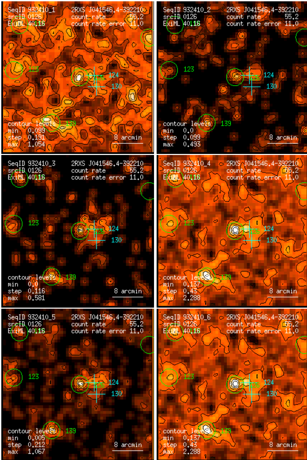
Figure 126: RASS 932410: detection 0126: band rate images, Gaussian filter: (1) PSPC channels 11 – 41, (2) 52 – 90, (3) 91 – 201, (4) 11 – 235, (5) 52 – 201, (6) 11 – 201. Broad band rates in counts/ks. Band rate contour levels in counts/ks/arcmin 2 .
