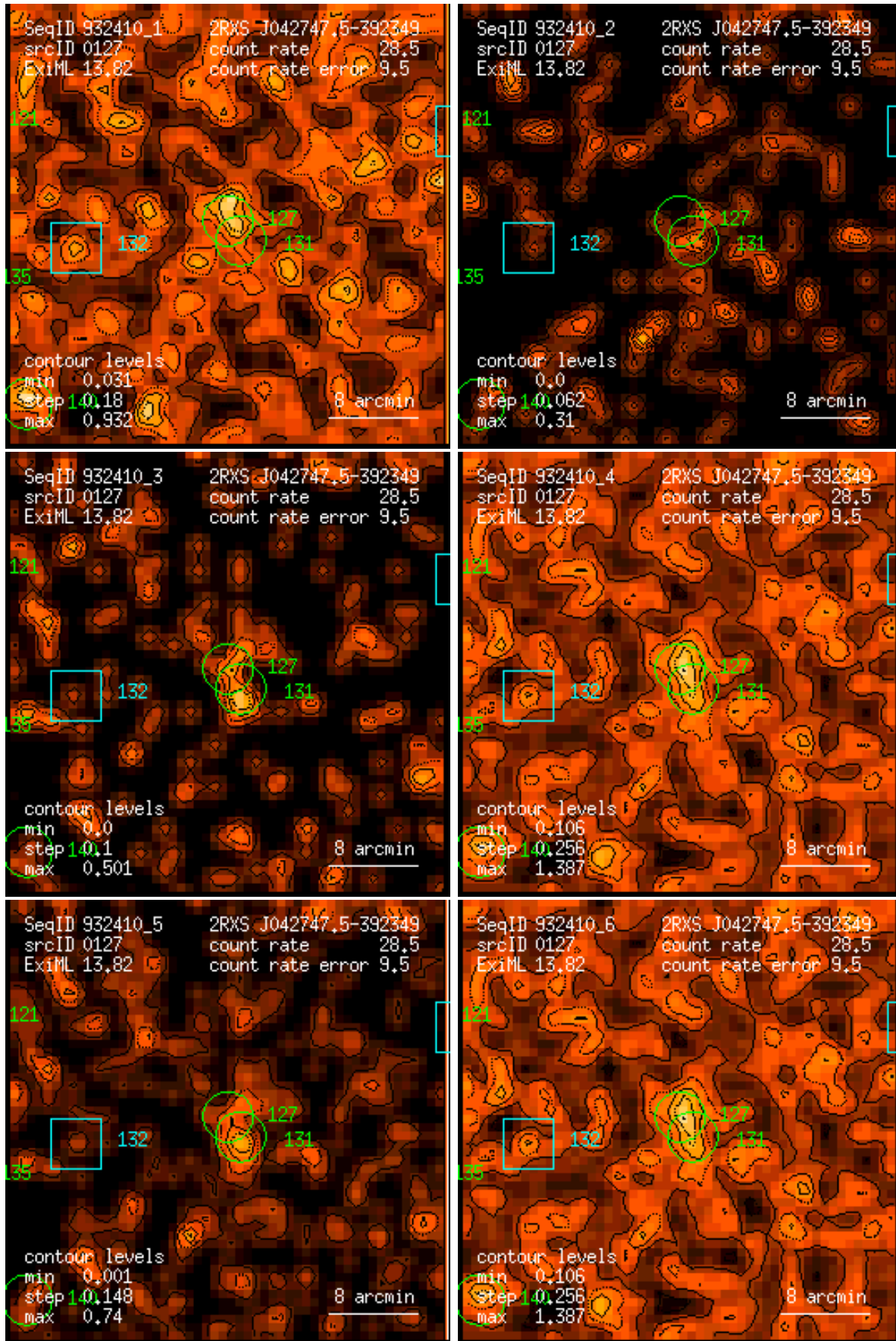
Figure 127: RASS 932410: detection 0127: band rate images, Gaussian filter: (1) PSPC channels 11 – 41, (2) 52 – 90, (3) 91 – 201, (4) 11 – 235, (5) 52 – 201, (6) 11 – 201. Broad band rates in counts/ks. Band rate contour levels in counts/ks/arcmin 2 .
