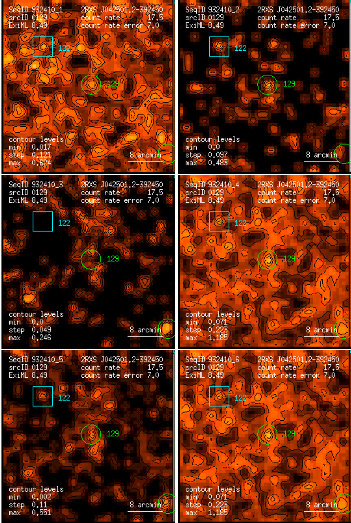
Figure 129: RASS 932410: detection 0129: band rate images, Gaussian filter: (1) PSPC channels 11 – 41, (2) 52 – 90, (3) 91 – 201, (4) 11 – 235, (5) 52 – 201, (6) 11 – 201. Broad band rates in counts/ks. Band rate contour levels in counts/ks/arcmin 2 .
