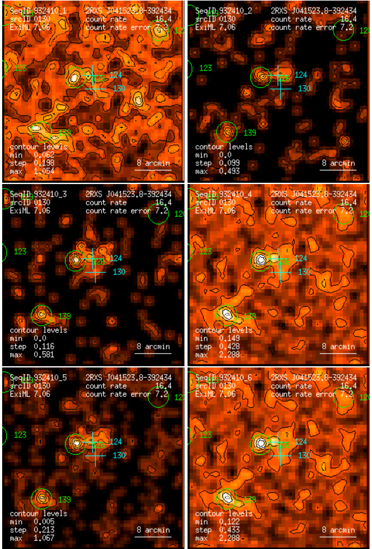
Figure 130: RASS 932410: detection 0130: band rate images, Gaussian filter: (1) PSPC channels 11 – 41, (2) 52 – 90, (3) 91 – 201, (4) 11 – 235, (5) 52 – 201, (6) 11 – 201. Broad band rates in counts/ks. Band rate contour levels in counts/ks/arcmin 2 .
