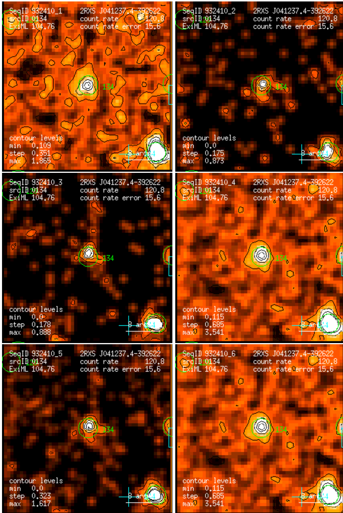
Figure 134: RASS 932410: detection 0134: band rate images, Gaussian filter: (1) PSPC channels 11 – 41, (2) 52 – 90, (3) 91 – 201, (4) 11 – 235, (5) 52 – 201, (6) 11 – 201. Broad band rates in counts/ks. Band rate contour levels in counts/ks/arcmin 2 .
