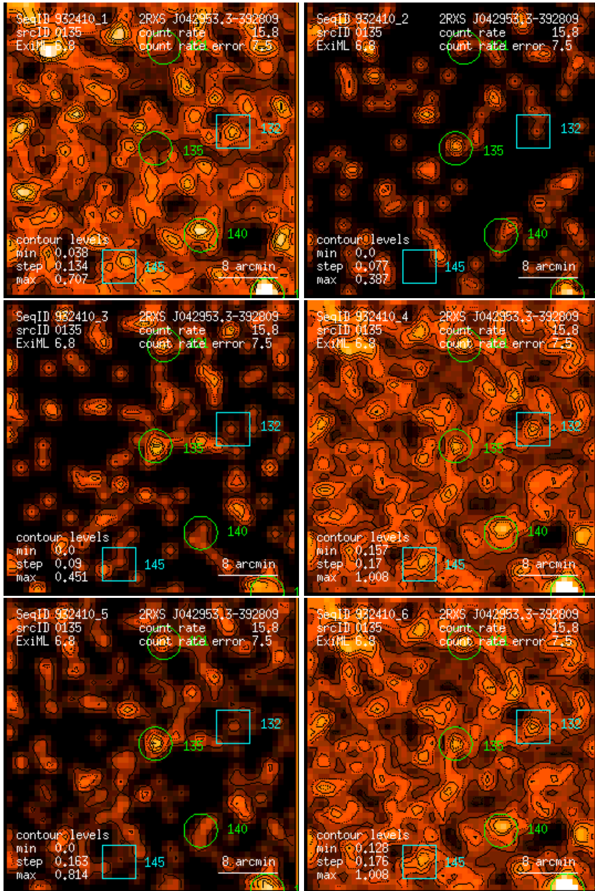
Figure 135: RASS 932410: detection 0135: band rate images, Gaussian filter: (1) PSPC channels 11 – 41, (2) 52 – 90, (3) 91 – 201, (4) 11 – 235, (5) 52 – 201, (6) 11 – 201. Broad band rates in counts/ks. Band rate contour levels in counts/ks/arcmin 2 .
