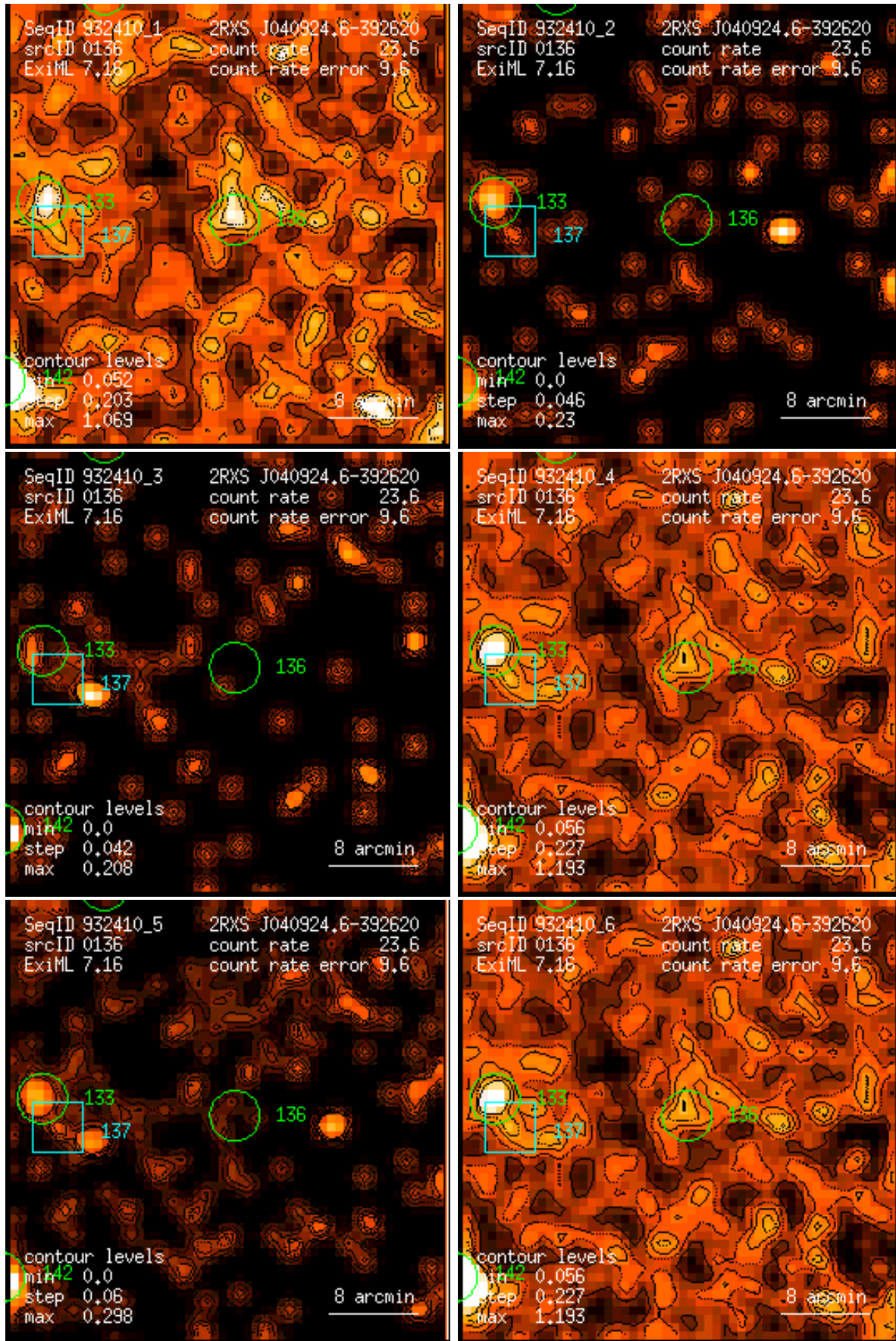
Figure 136: RASS 932410: detection 0136: band rate images, Gaussian filter: (1) PSPC channels 11 – 41, (2) 52 – 90, (3) 91 – 201, (4) 11 – 235, (5) 52 – 201, (6) 11 – 201. Broad band rates in counts/ks. Band rate contour levels in counts/ks/arcmin 2 .
