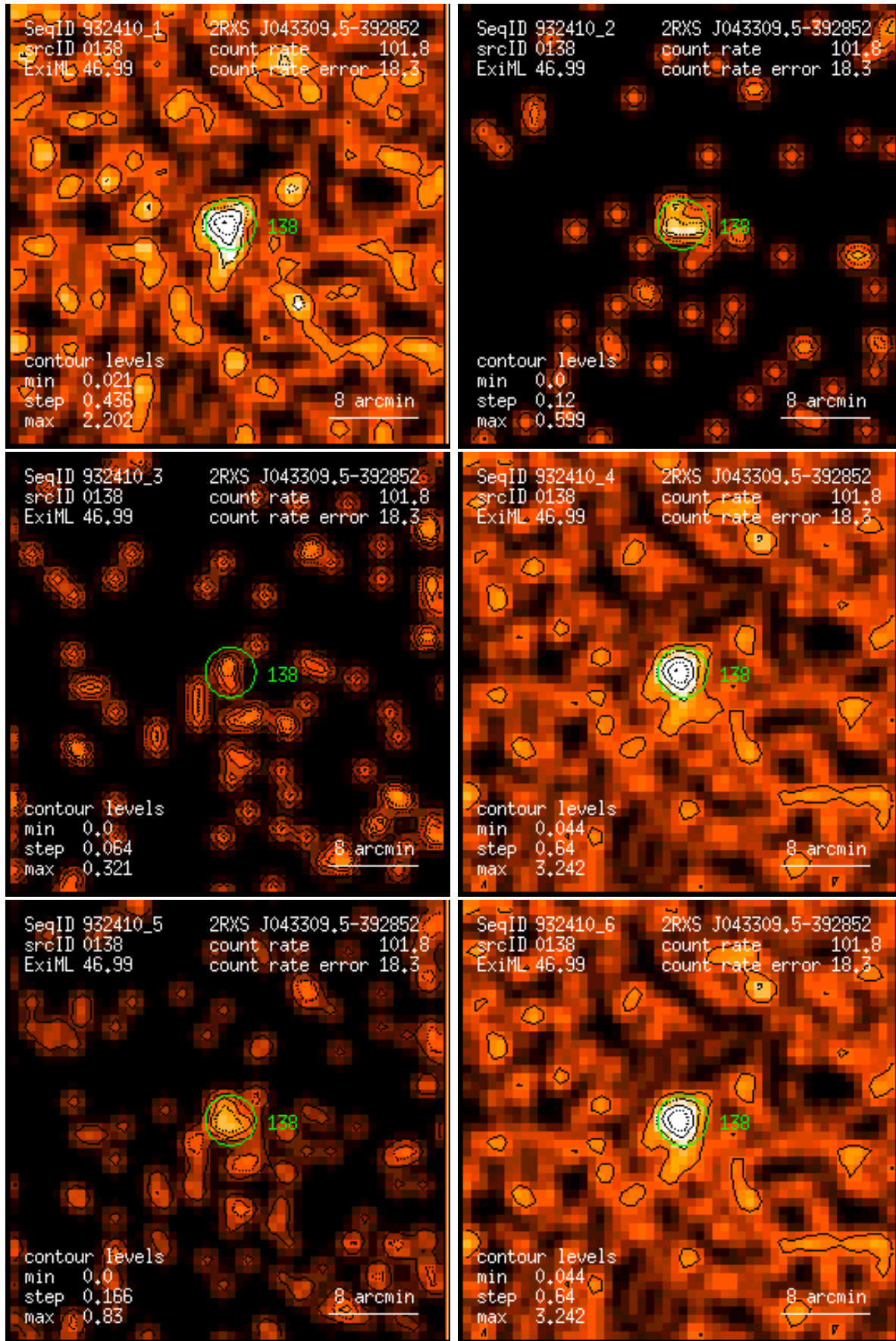
Figure 138: RASS 932410: detection 0138: band rate images, Gaussian filter: (1) PSPC channels 11 – 41, (2) 52 – 90, (3) 91 – 201, (4) 11 – 235, (5) 52 – 201, (6) 11 – 201. Broad band rates in counts/ks. Band rate contour levels in counts/ks/arcmin 2 .
