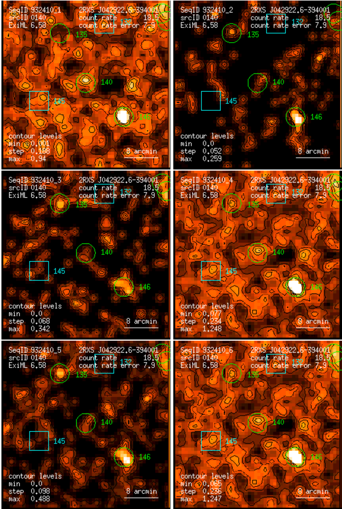
Figure 140: RASS 932410: detection 0140: band rate images, Gaussian filter: (1) PSPC channels 11 – 41, (2) 52 – 90, (3) 91 – 201, (4) 11 – 235, (5) 52 – 201, (6) 11 – 201. Broad band rates in counts/ks. Band rate contour levels in counts/ks/arcmin 2 .
