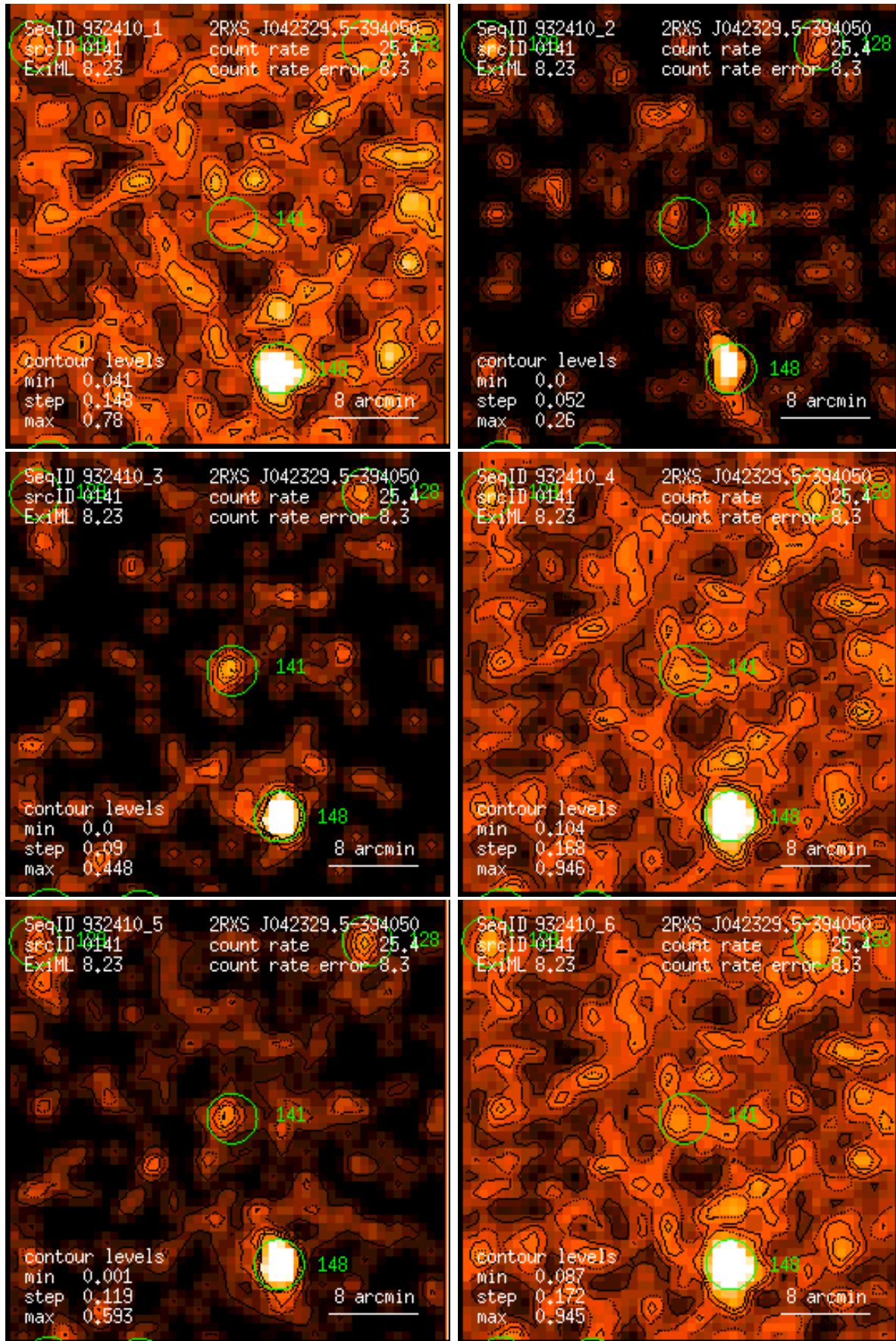
Figure 141: RASS 932410: detection 0141: band rate images, Gaussian filter: (1) PSPC channels 11 – 41, (2) 52 – 90, (3) 91 – 201, (4) 11 – 235, (5) 52 – 201, (6) 11 – 201. Broad band rates in counts/ks. Band rate contour levels in counts/ks/arcmin 2 .
