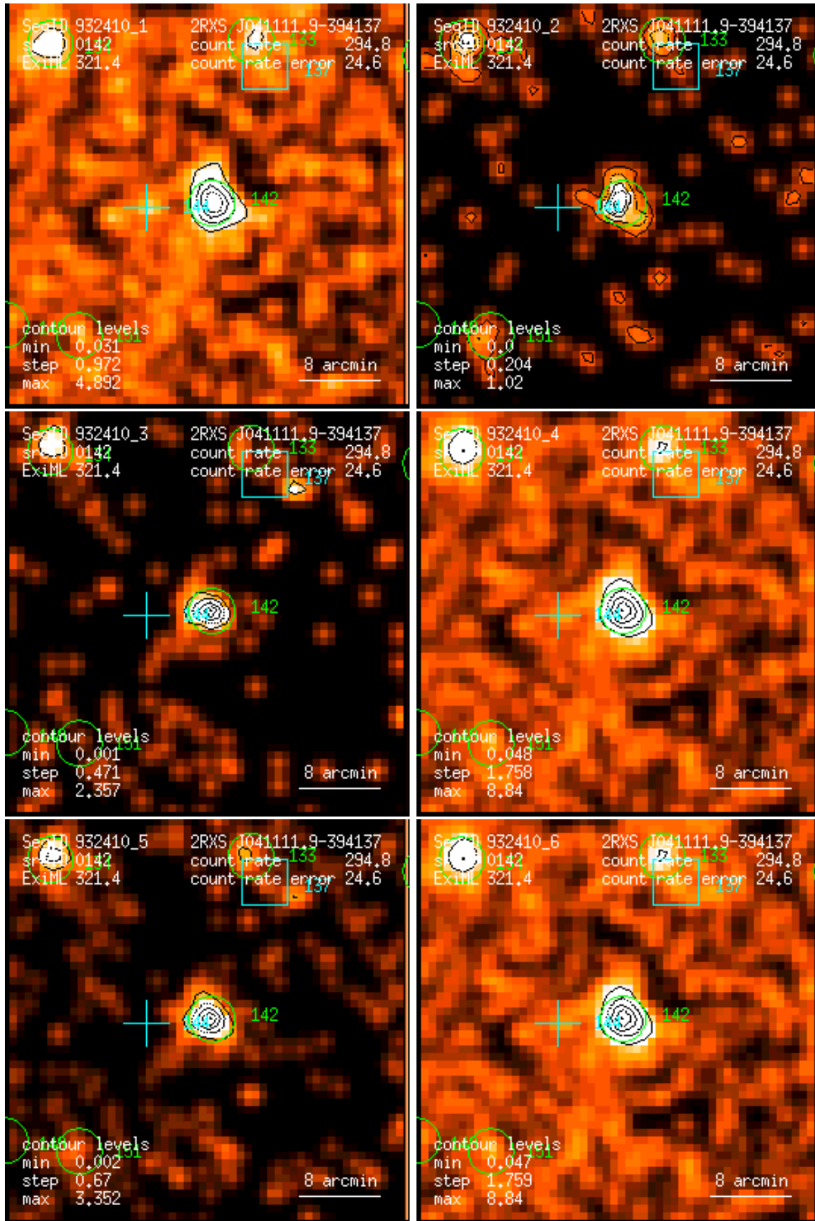
Figure 142: RASS 932410: detection 0142: band rate images, Gaussian filter: (1) PSPC channels 11 – 41, (2) 52 – 90, (3) 91 – 201, (4) 11 – 235, (5) 52 – 201, (6) 11 – 201. Broad band rates in counts/ks. Band rate contour levels in counts/ks/arcmin 2 .
