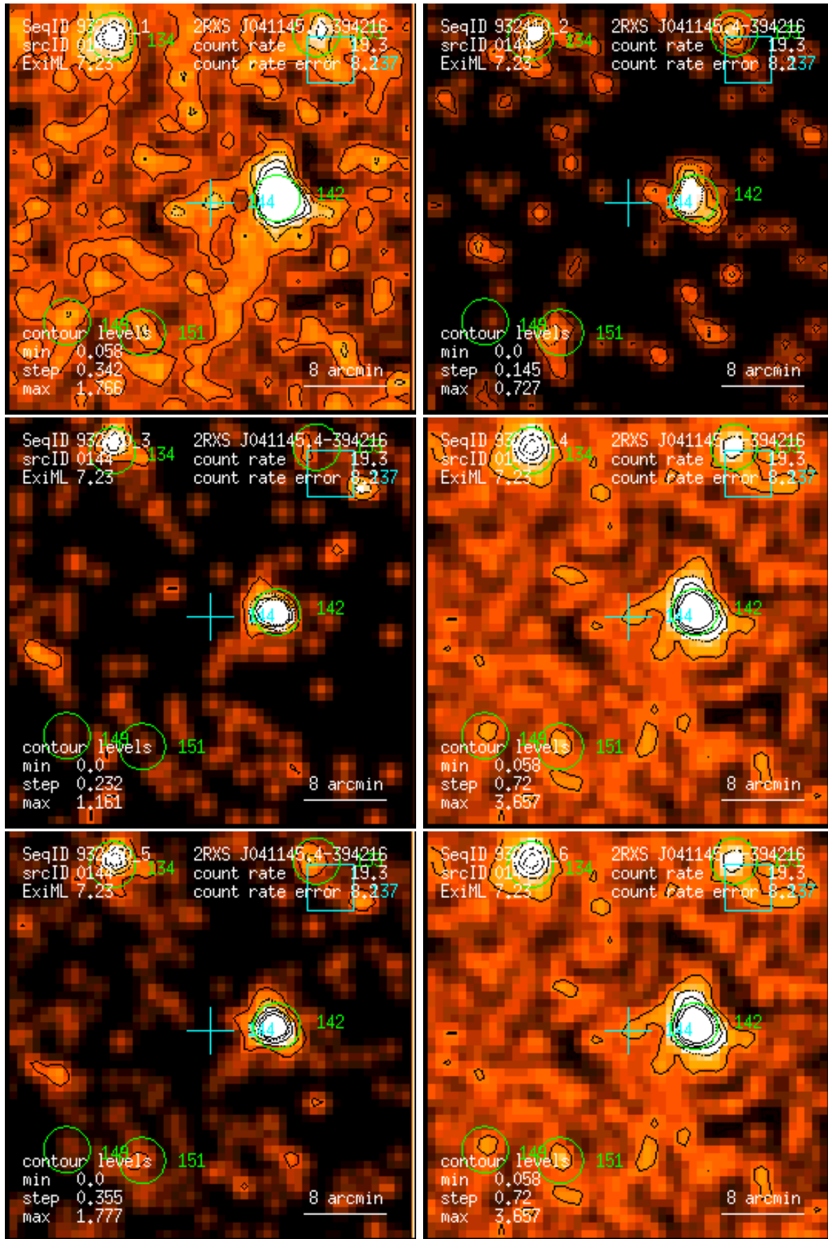
Figure 144: RASS 932410: detection 0144: band rate images, Gaussian filter: (1) PSPC channels 11 – 41, (2) 52 – 90, (3) 91 – 201, (4) 11 – 235, (5) 52 – 201, (6) 11 – 201. Broad band rates in counts/ks. Band rate contour levels in counts/ks/arcmin 2 .
