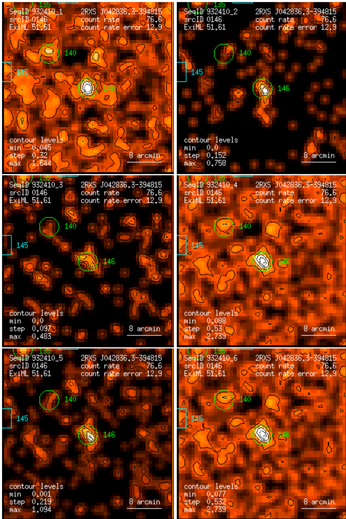
Figure 146: RASS 932410: detection 0146: band rate images, Gaussian filter: (1) PSPC channels 11 – 41, (2) 52 – 90, (3) 91 – 201, (4) 11 – 235, (5) 52 – 201, (6) 11 – 201. Broad band rates in counts/ks. Band rate contour levels in counts/ks/arcmin 2 .
