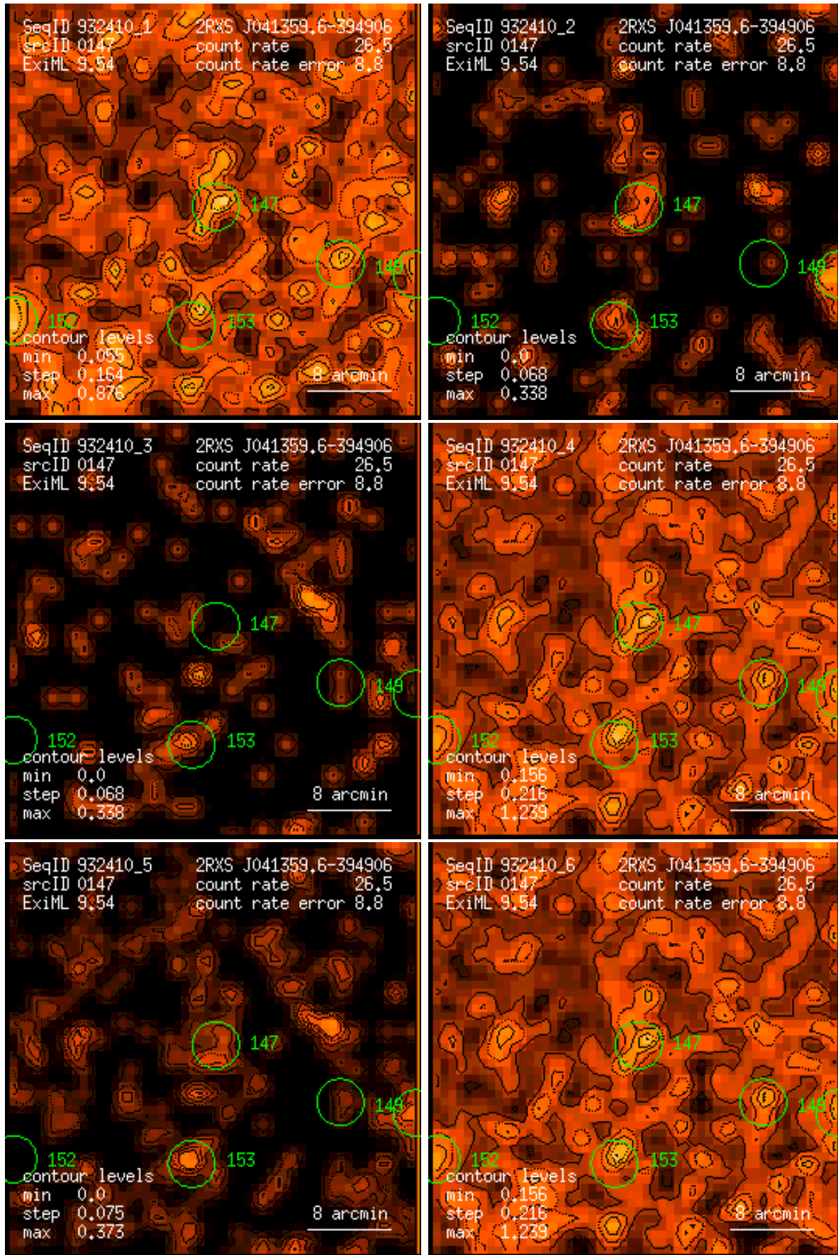
Figure 147: RASS 932410: detection 0147: band rate images, Gaussian filter: (1) PSPC channels 11 – 41, (2) 52 – 90, (3) 91 – 201, (4) 11 – 235, (5) 52 – 201, (6) 11 – 201. Broad band rates in counts/ks. Band rate contour levels in counts/ks/arcmin 2 .
