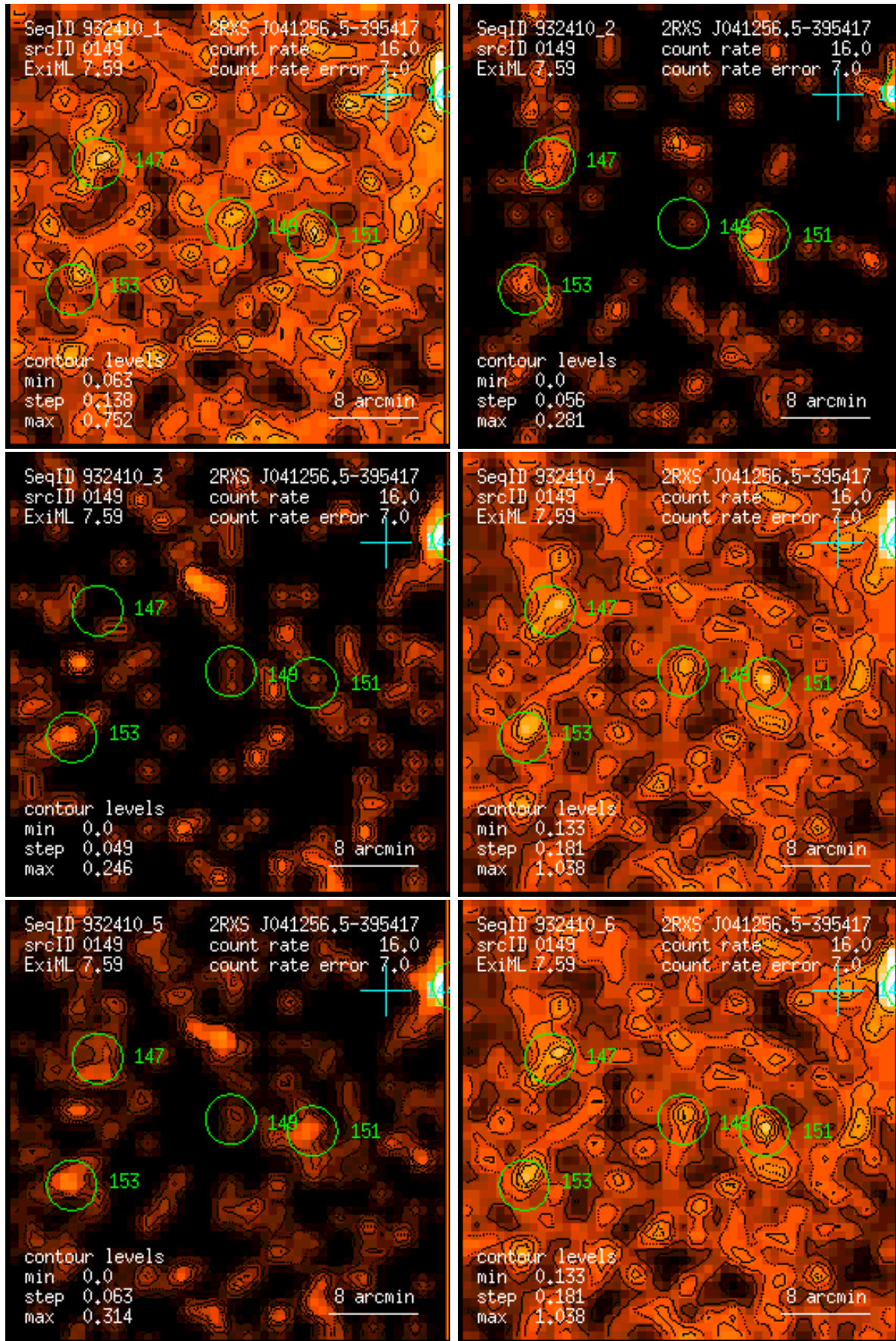
Figure 149: RASS 932410: detection 0149: band rate images, Gaussian filter: (1) PSPC channels 11 – 41, (2) 52 – 90, (3) 91 – 201, (4) 11 – 235, (5) 52 – 201, (6) 11 – 201. Broad band rates in counts/ks. Band rate contour levels in counts/ks/arcmin 2 .
