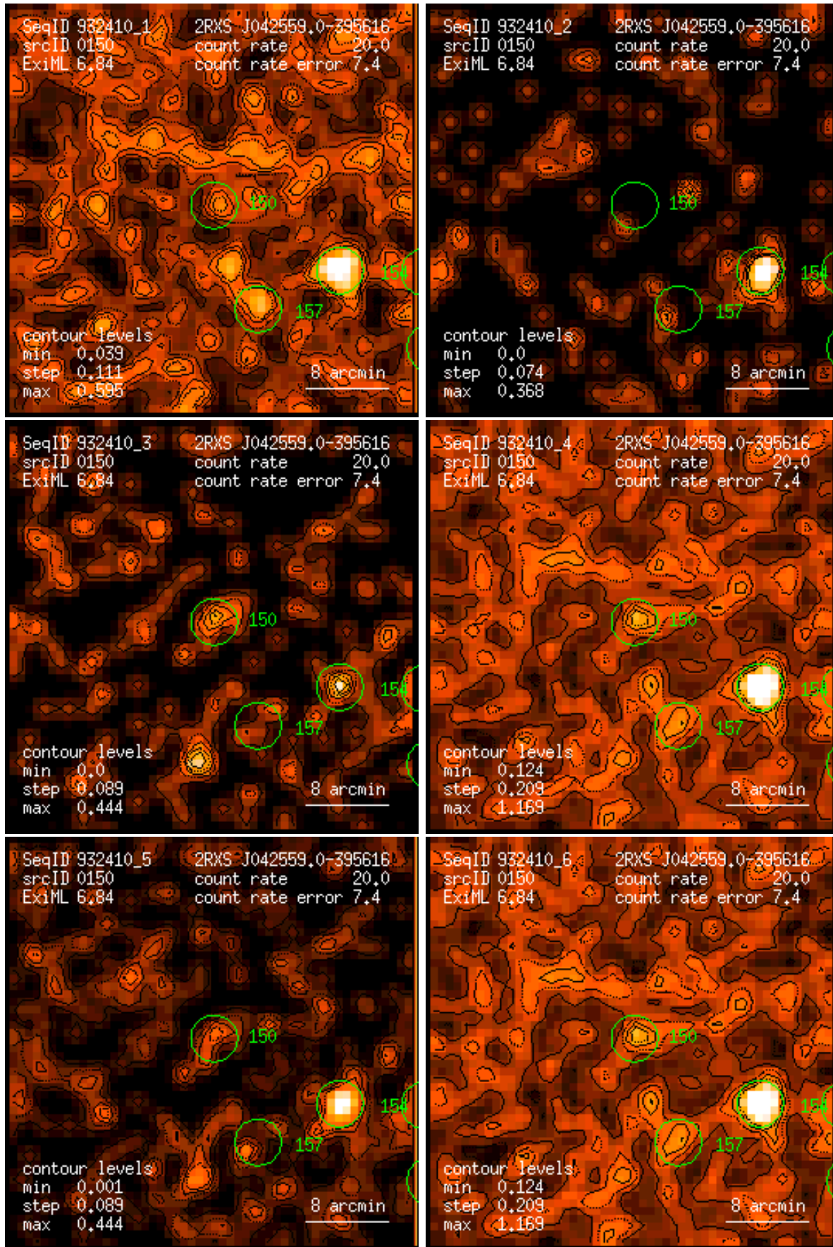
Figure 150: RASS 932410: detection 0150: band rate images, Gaussian filter: (1) PSPC channels 11 – 41, (2) 52 – 90, (3) 91 – 201, (4) 11 – 235, (5) 52 – 201, (6) 11 – 201. Broad band rates in counts/ks. Band rate contour levels in counts/ks/arcmin 2 .
