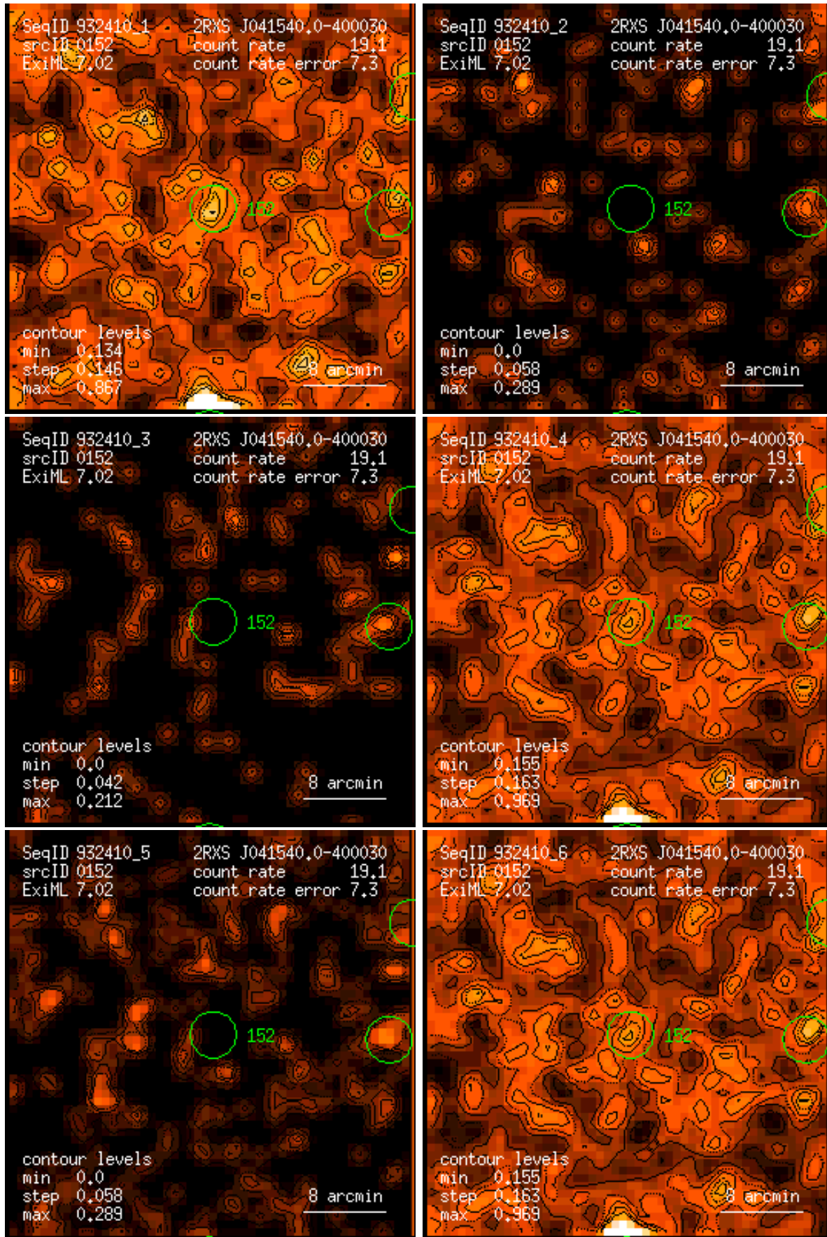
Figure 152: RASS 932410: detection 0152: band rate images, Gaussian filter: (1) PSPC channels 11 – 41, (2) 52 – 90, (3) 91 – 201, (4) 11 – 235, (5) 52 – 201, (6) 11 – 201. Broad band rates in counts/ks. Band rate contour levels in counts/ks/arcmin 2 .
