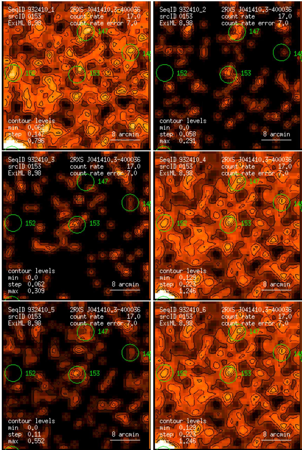
Figure 153: RASS 932410: detection 0153: band rate images, Gaussian filter: (1) PSPC channels 11 – 41, (2) 52 – 90, (3) 91 – 201, (4) 11 – 235, (5) 52 – 201, (6) 11 – 201. Broad band rates in counts/ks. Band rate contour levels in counts/ks/arcmin 2 .
