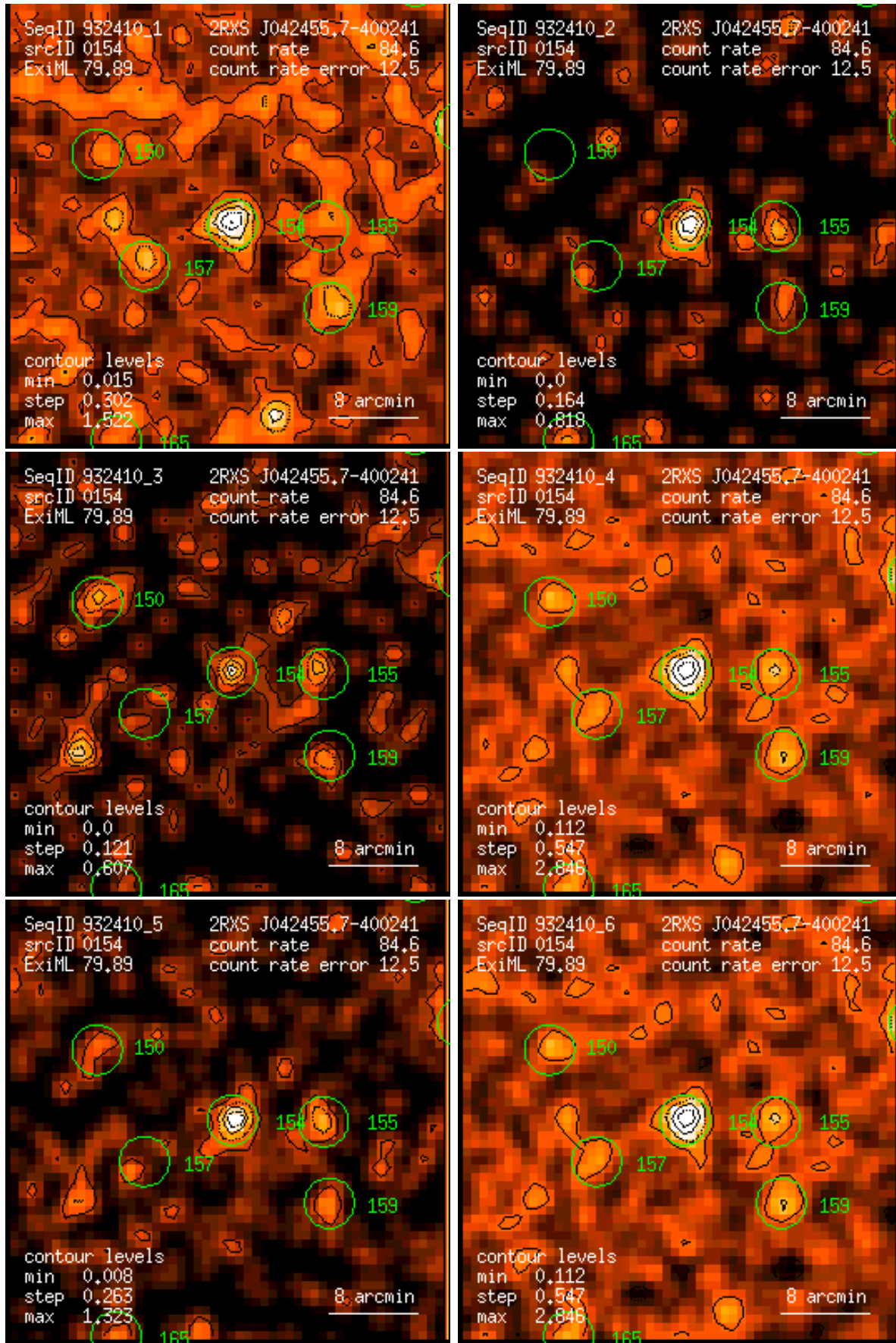
Figure 154: RASS 932410: detection 0154: band rate images, Gaussian filter: (1) PSPC channels 11 – 41, (2) 52 – 90, (3) 91 – 201, (4) 11 – 235, (5) 52 – 201, (6) 11 – 201. Broad band rates in counts/ks. Band rate contour levels in counts/ks/arcmin 2 .
