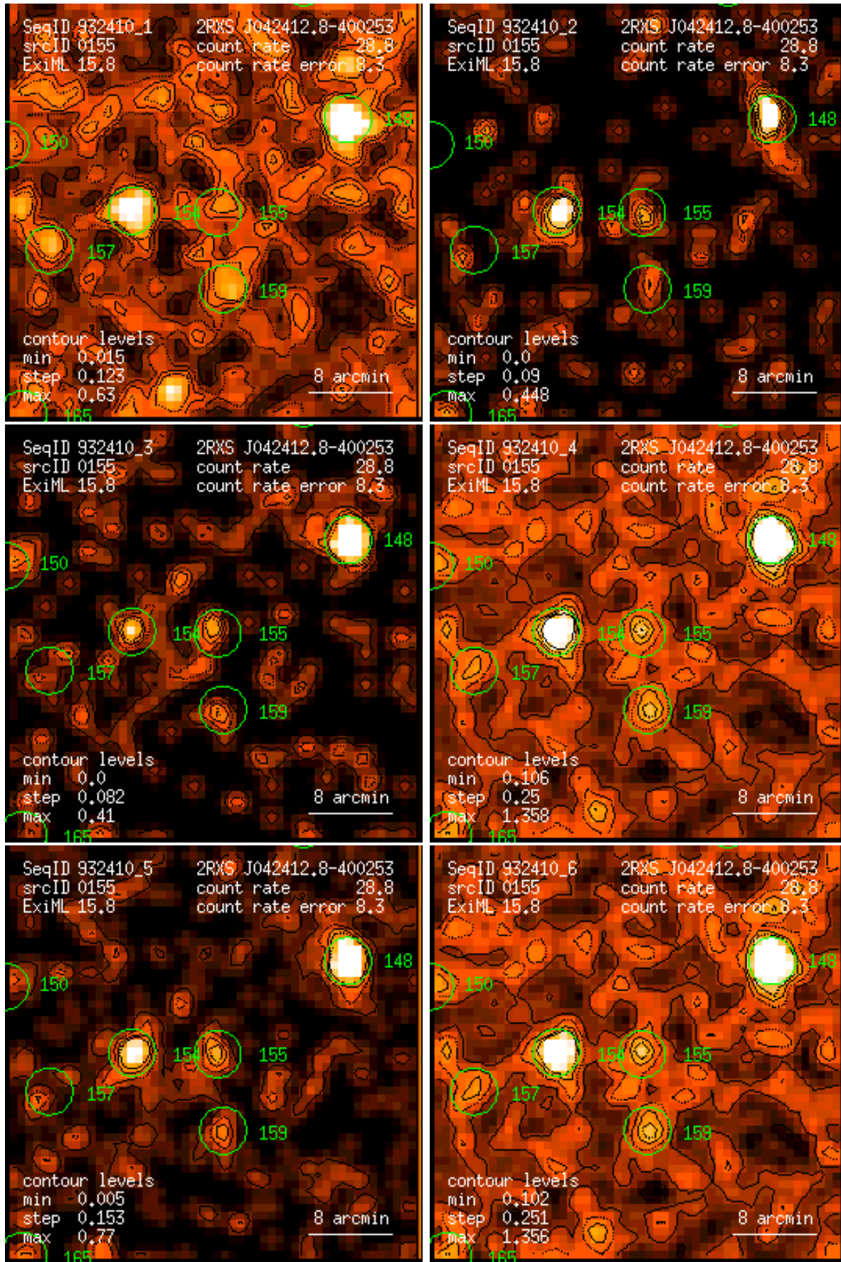
Figure 155: RASS 932410: detection 0155: band rate images, Gaussian filter: (1) PSPC channels 11 – 41, (2) 52 – 90, (3) 91 – 201, (4) 11 – 235, (5) 52 – 201, (6) 11 – 201. Broad band rates in counts/ks. Band rate contour levels in counts/ks/arcmin 2 .
