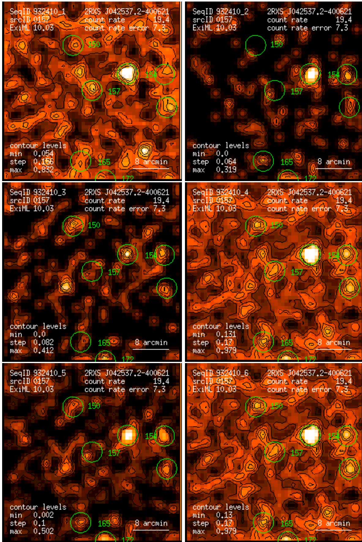
Figure 157: RASS 932410: detection 0157: band rate images, Gaussian filter: (1) PSPPC channels 11 – 41, (2) 52 – 90, (3) 91 – 201, (4) 11 – 235, (5) 52 – 201, (6) 11 – 201. Broad band rates in counts/ks. Band rate contour levels in counts/ks/arcmin 2 .
