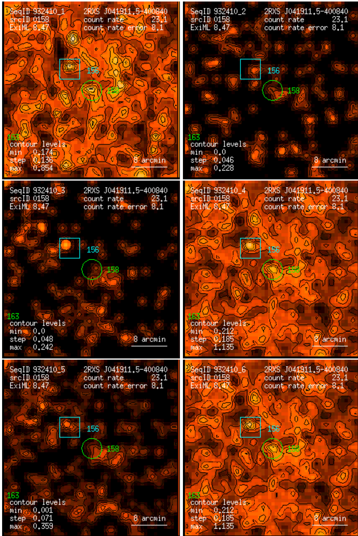
Figure 158: RASS 932410: detection 0158: band rate images, Gaussian filter: (1) PSPC channels 11 – 41, (2) 52 – 90, (3) 91 – 201, (4) 11 – 235, (5) 52 – 201, (6) 11 – 201. Broad band rates in counts/ks. Band rate contour levels in counts/ks/arcmin 2 .
