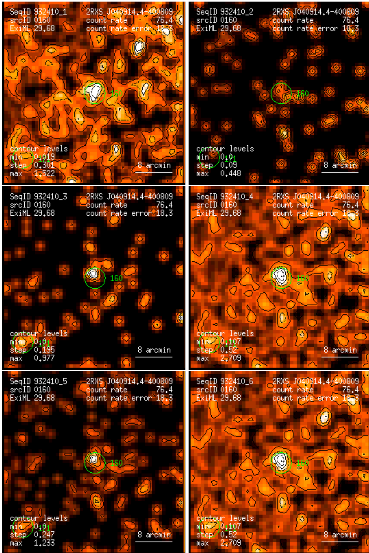
Figure 160: RASS 932410: detection 0160: band rate images, Gaussian filter: (1) PSPC channels 11 – 41, (2) 52 – 90, (3) 91 – 201, (4) 11 – 235, (5) 52 – 201, (6) 11 – 201. Broad band rates in counts/ks. Band rate contour levels in counts/ks/arcmin 2 .
