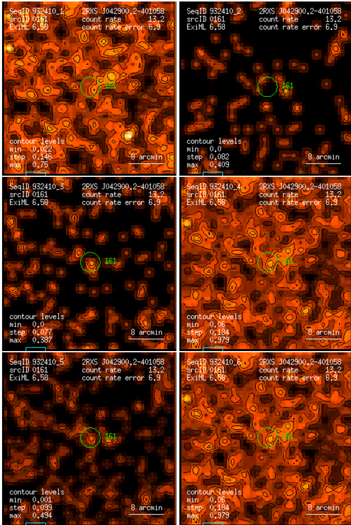
Figure 161: RASS 932410: detection 0161: band rate images, Gaussian filter: (1) PSPC channels 11 – 41, (2) 52 – 90, (3) 91 – 201, (4) 11 – 235, (5) 52 – 201, (6) 11 – 201. Broad band rates in counts/ks. Band rate contour levels in counts/ks/arcmin 2 .
