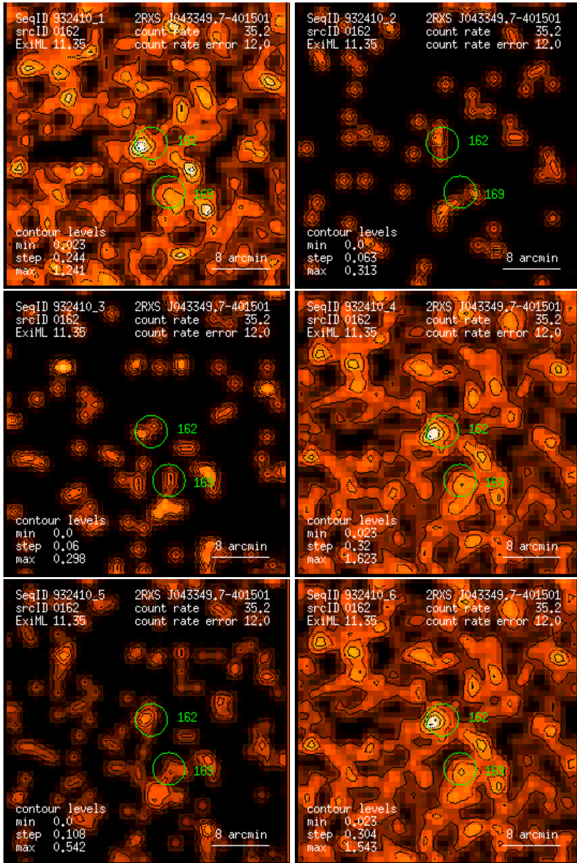
Figure 162: RASS 932410: detection 0162: band rate images, Gaussian filter: (1) PSPC channels 11 – 41, (2) 52 – 90, (3) 91 – 201, (4) 11 – 235, (5) 52 – 201, (6) 11 – 201. Broad band rates in counts/ks. Band rate contour levels in counts/ks/arcmin 2 .
