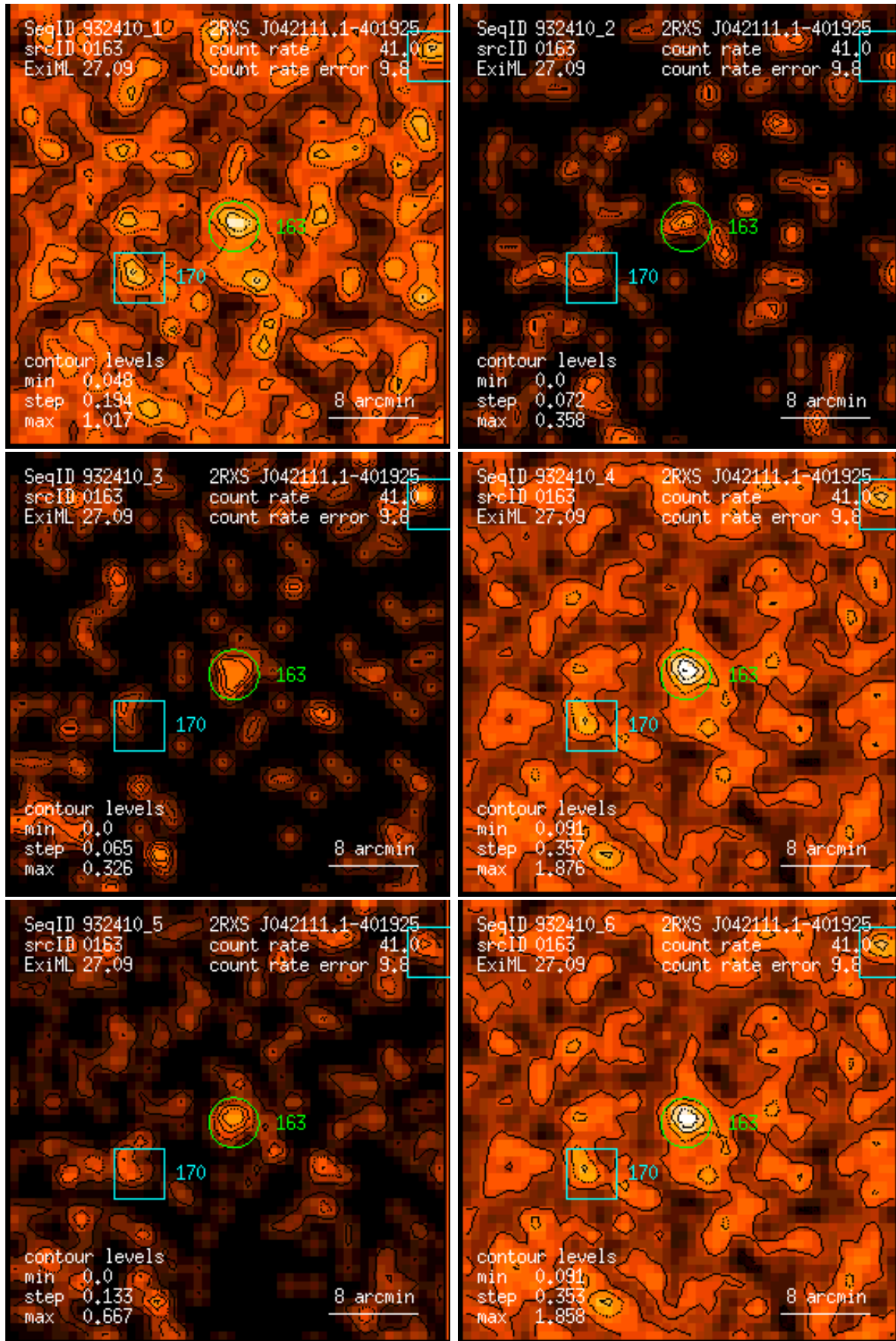
Figure 163: RASS 932410: detection 0163: band rate images, Gaussian filter: (1) PSPC channels 11 – 41, (2) 52 – 90, (3) 91 – 201, (4) 11 – 235, (5) 52 – 201, (6) 11 – 201. Broad band rates in counts/ks. Band rate contour levels in counts/ks/arcmin 2 .
