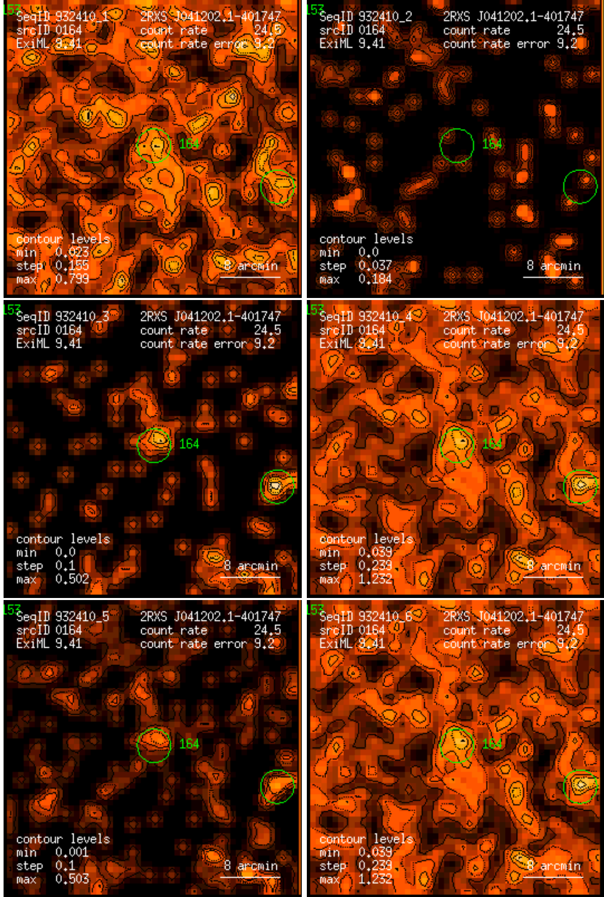
Figure 164: RASS 932410: detection 0164: band rate images, Gaussian filter: (1) PSPC channels 11 – 41, (2) 52 – 90, (3) 91 – 201, (4) 11 – 235, (5) 52 – 201, (6) 11 – 201. Broad band rates in counts/ks. Band rate contour levels in counts/ks/arcmin 2 .
