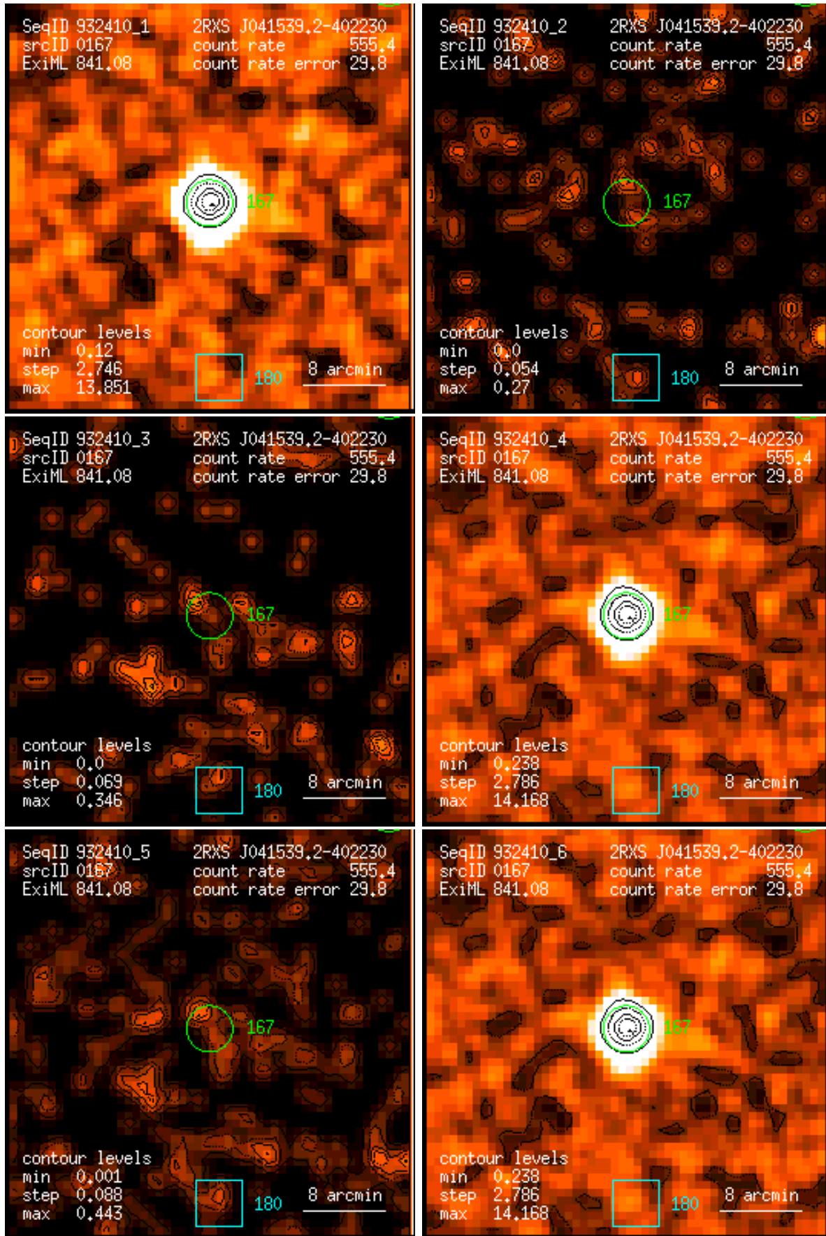
Figure 167: RASS 932410: detection 0167: band rate images, Gaussian filter: (1) PSPC channels 11 – 41, (2) 52 – 90, (3) 91 – 201, (4) 11 – 235, (5) 52 – 201, (6) 11 – 201. Broad band rates in counts/ks. Band rate contour levels in counts/ks/arcmin 2 .
