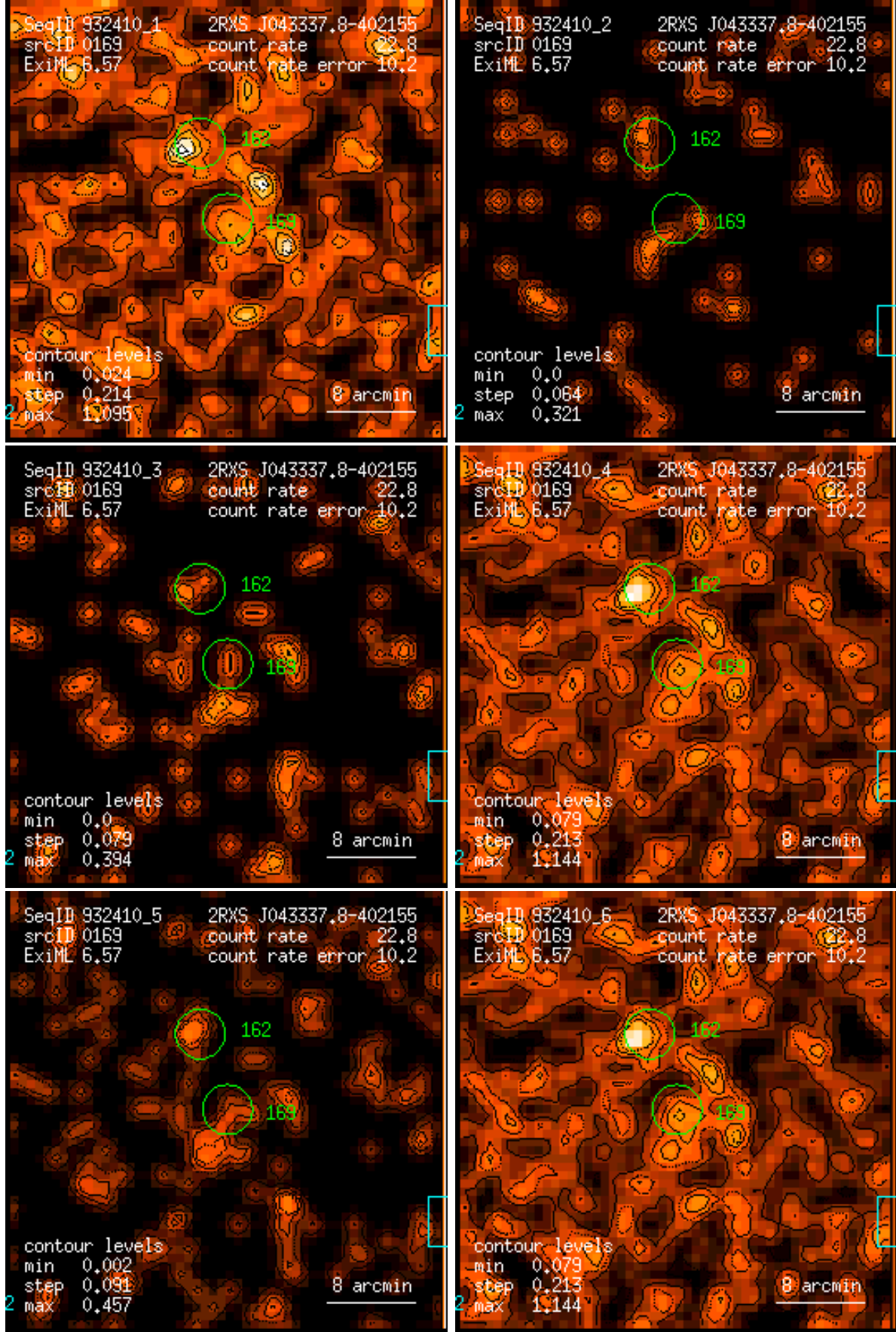
Figure 169: RASS 932410: detection 0169: band rate images, Gaussian filter: (1) PSPC channels 11 – 41, (2) 52 – 90, (3) 91 – 201, (4) 11 – 235, (5) 52 – 201, (6) 11 – 201. Broad band rates in counts/ks. Band rate contour levels in counts/ks/arcmin 2 .
