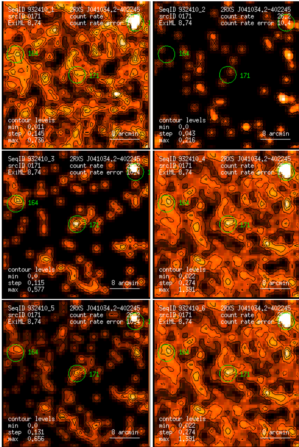
Figure 171: RASS 932410: detection 0171: band rate images, Gaussian filter: (1) PSPC channels 11 – 41, (2) 52 – 90, (3) 91 – 201, (4) 11 – 235, (5) 52 – 201, (6) 11 – 201. Broad band rates in counts/ks. Band rate contour levels in counts/ks/arcmin 2 .
