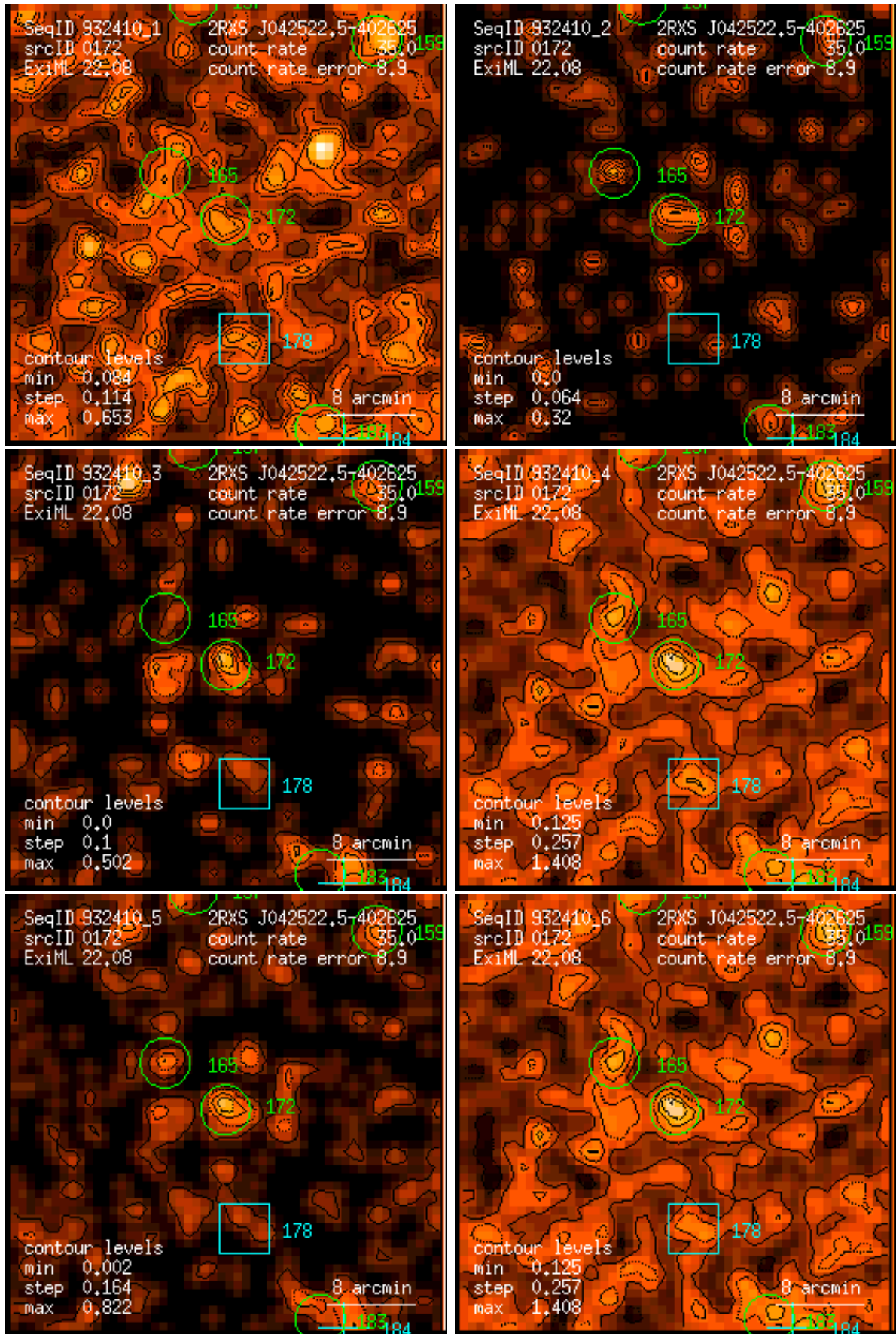
Figure 172: RASS 932410: detection 0172: band rate images, Gaussian filter: (1) PSPC channels 11 – 41, (2) 52 – 90, (3) 91 – 201, (4) 11 – 235, (5) 52 – 201, (6) 11 – 201. Broad band rates in counts/ks. Band rate contour levels in counts/ks/arcmin 2 .
